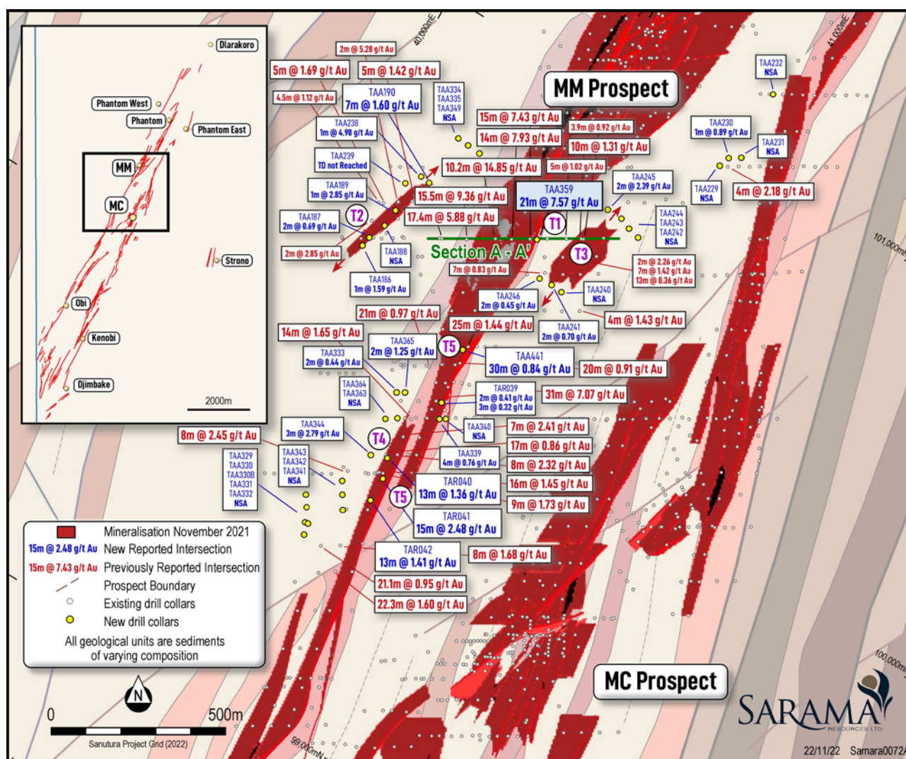
Figure 2 - MM Prospect – Plan of Mineralisation & Intersections Around Recent Drilling
