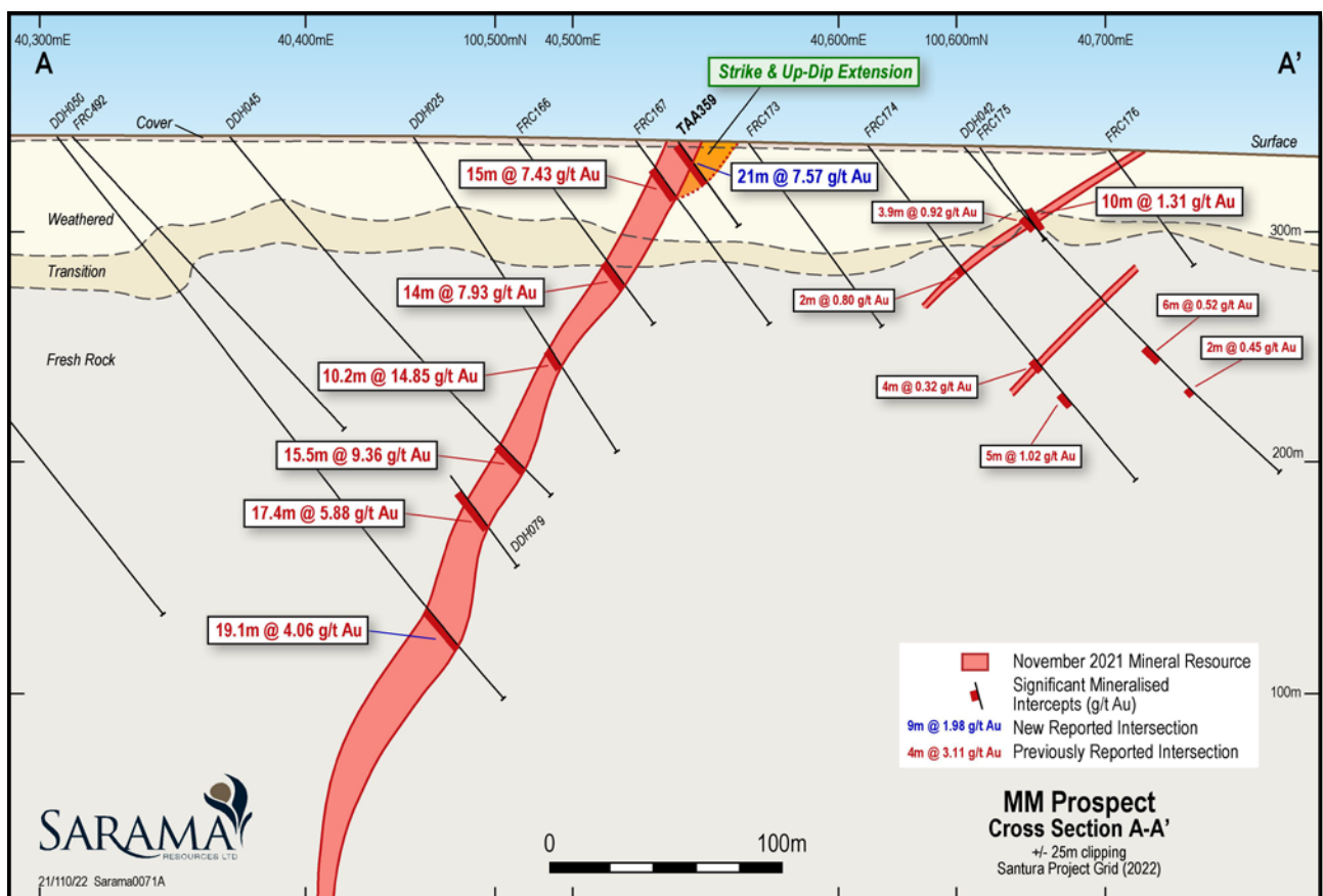
Figure 3 – High-Grade Oxide Mineralisation Intersected at T1 (Cross Section A-A' - Looking NNE)
