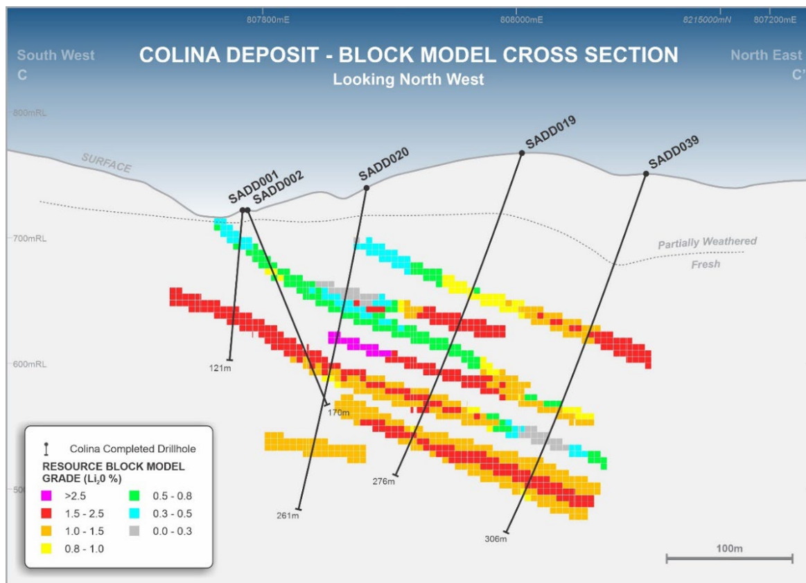
Figure 6: Colina MRE Block Model Cross Section C-C' (see Figure 7 for section location)
