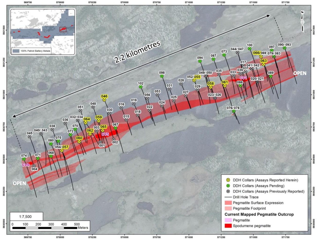
Figure 1: Drill hole collar locations at the CV5 Pegmatite for holes completed to date
