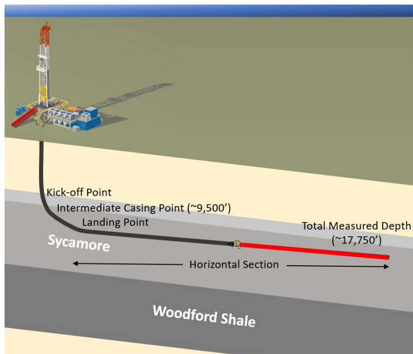
Figure1. Schematic - Wolf Pack Well
