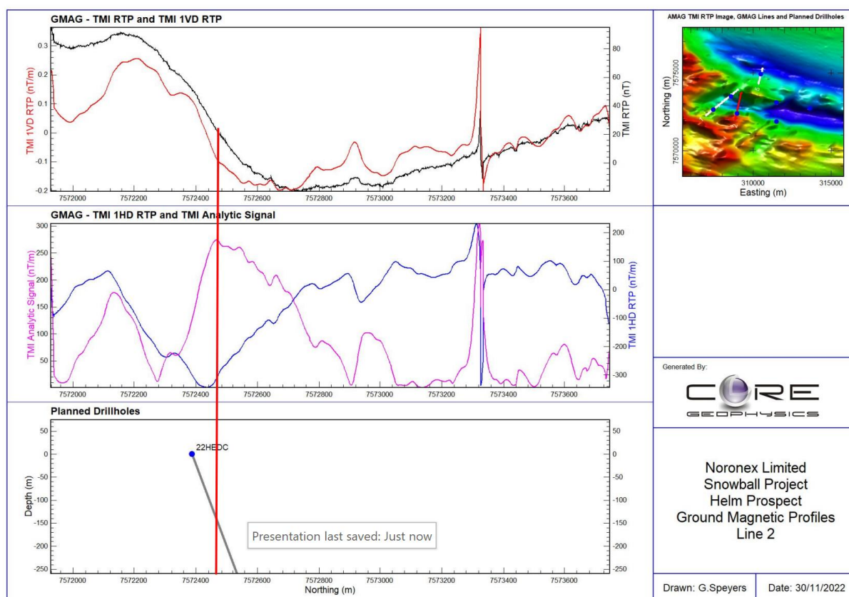
Figure 5. Ground magnetic profiles collected at Helm to target the antiformal structure and location of initial hole 22HED01.
