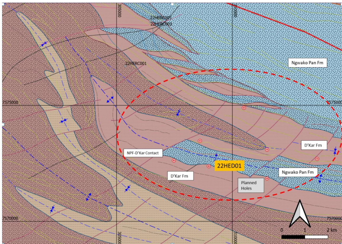
Figure 4. Helm targets outlined on a geological interpretation with initial hole 22HED01
