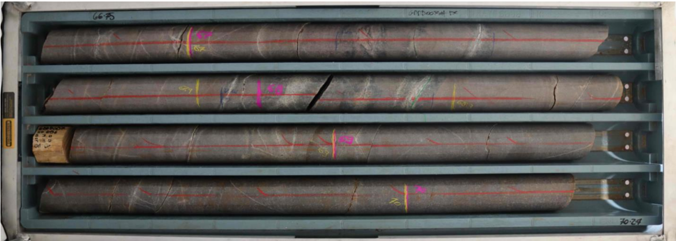
Figure 3. Quartz-sulphide veins, with alteration halo, in rhyolite ( 0.4m @ 18.0g/t Au from 67.9m).
