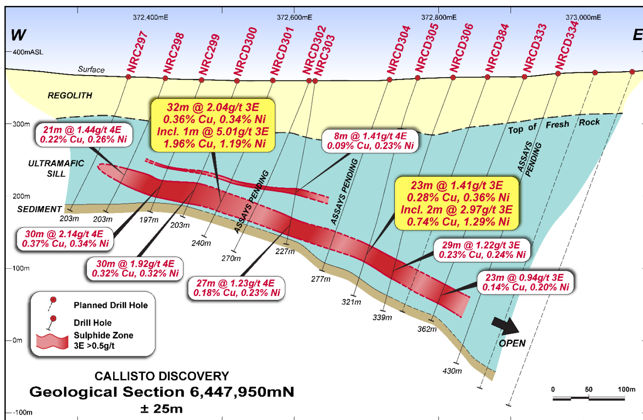
Figure 4 — Callisto geological interpretation section 6,447,950N showing broad zones of continuous mineralisation. Peak copper grades of 1.96%, with 2.62g/t Pd and 1.82 g/t Au, were recorded in NRCD301 (from 175m) within a broad 32 metre mineralised zone. See Appendices 1 and 2 for drill hole details. Mineralisation is open to the east.
