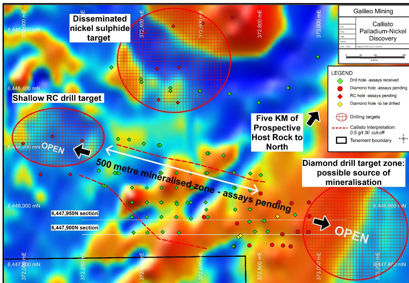
Figure 5 — Plan map of Callisto drilling with RC and diamond drill target zones. Red dashed lines show the interpreted mineralised zone at 0.5 g/t 3E cut-off projected to surface – open in both directions. 500 metre zone of mineralisation has been defined from assays received to date. Assays are pending for drilling to the east of the current mineralised zone. Source of mineralisation may exist to the east within diamond drill target zone as shown. Parent host rock (layered ultramafic sill) can be seen in the magnetic imagery striking to the north-northeast. Section lines in Figures 2 and 4. Background magnetic image is TMI-1VD.
