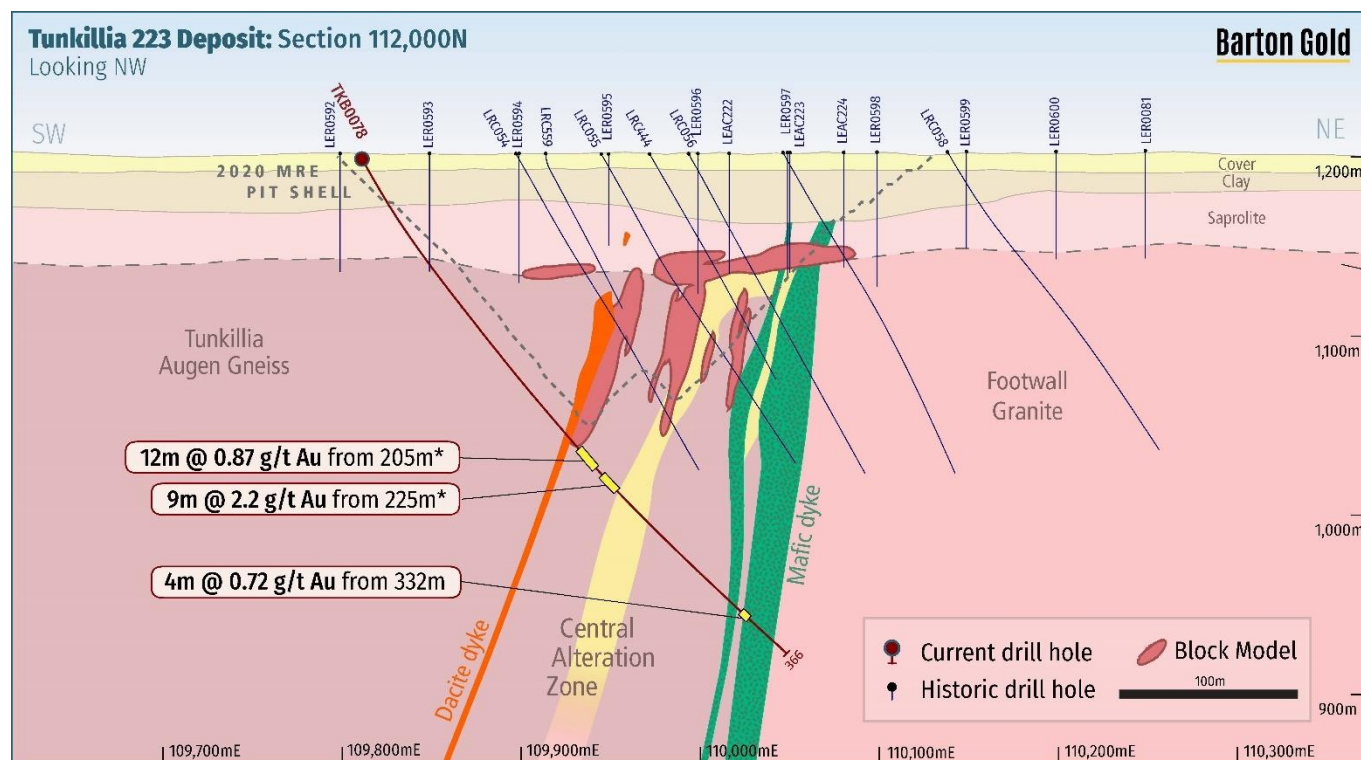
Figure 6 – Tunkillia RC Drill Hole TKB0078
