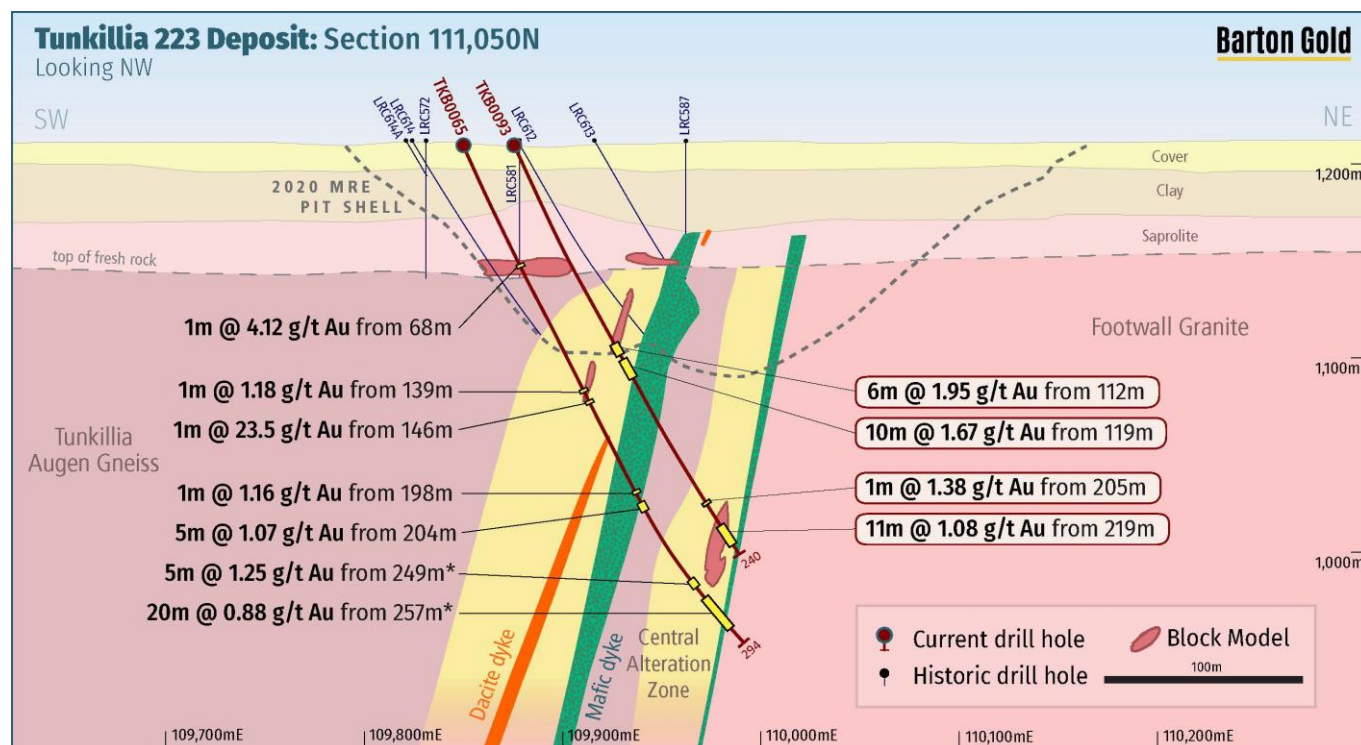
Figure 4 – Tunkillia RC Drill Holes TKB0065 (published 15 Dec 2022) & TKB0093
