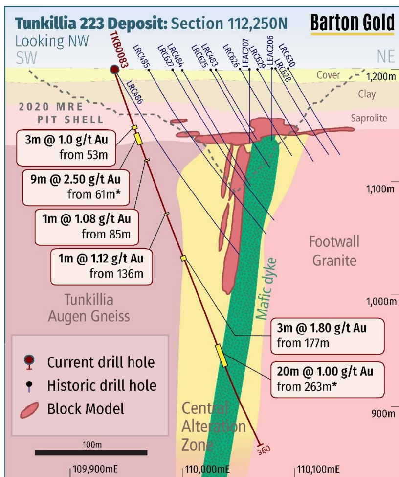
Figure 7 – Tunkillia RC Drill Hole TKB0083
