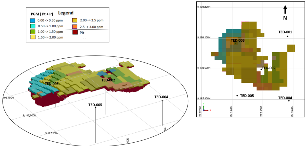
Figure 7: Tabocal Pit Optimisation result, Inferred resources
