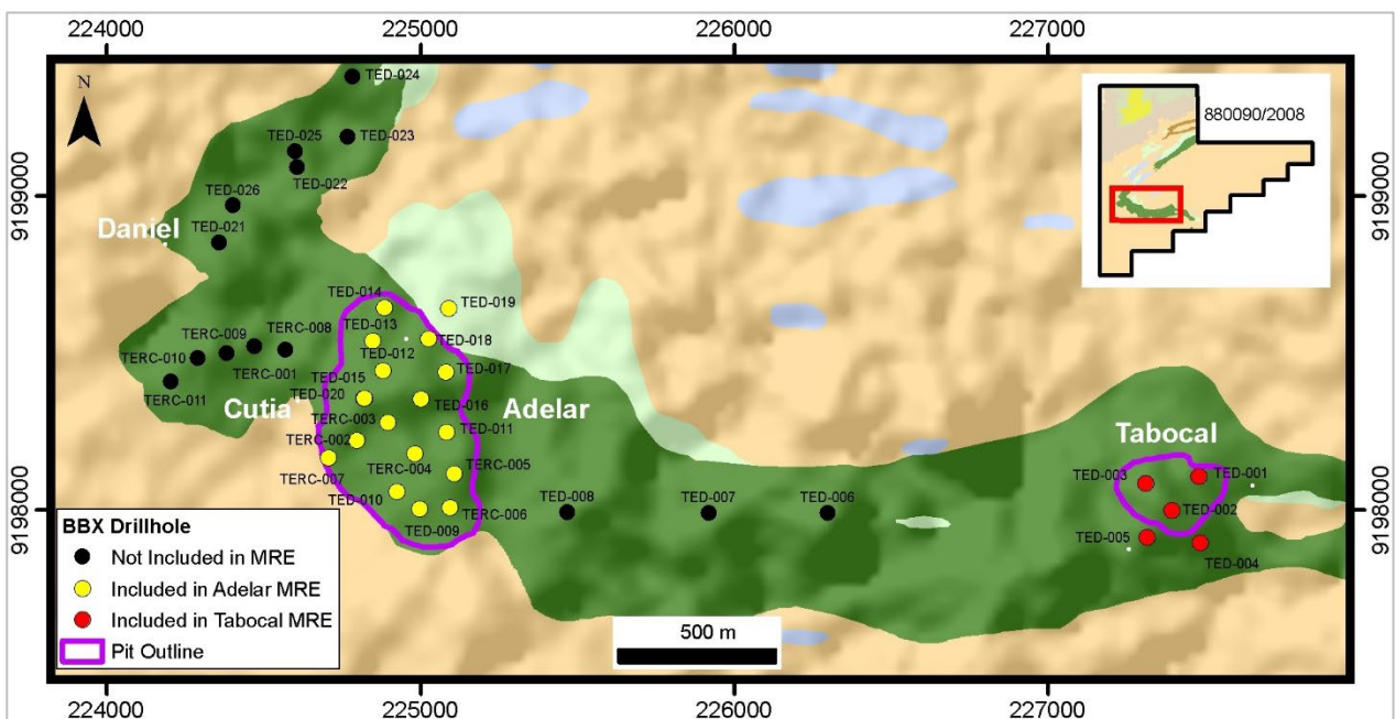
Figure 6: Adelar and Tabocal drill collar location
