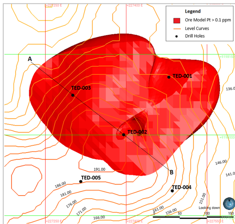
Figure 1: Tabocal target mineralised zone map
