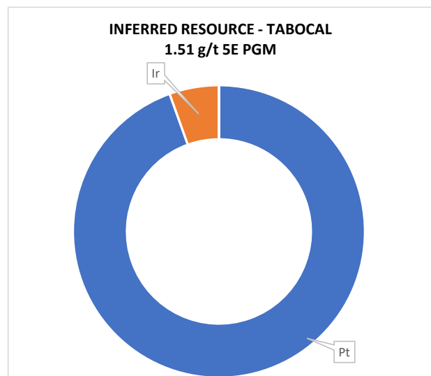
Figure 4: Inferred 5E PGM Resource (relative grade), Tabocal
