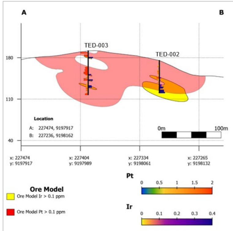
Figure 2: Tabocal target mineralised cross-section
