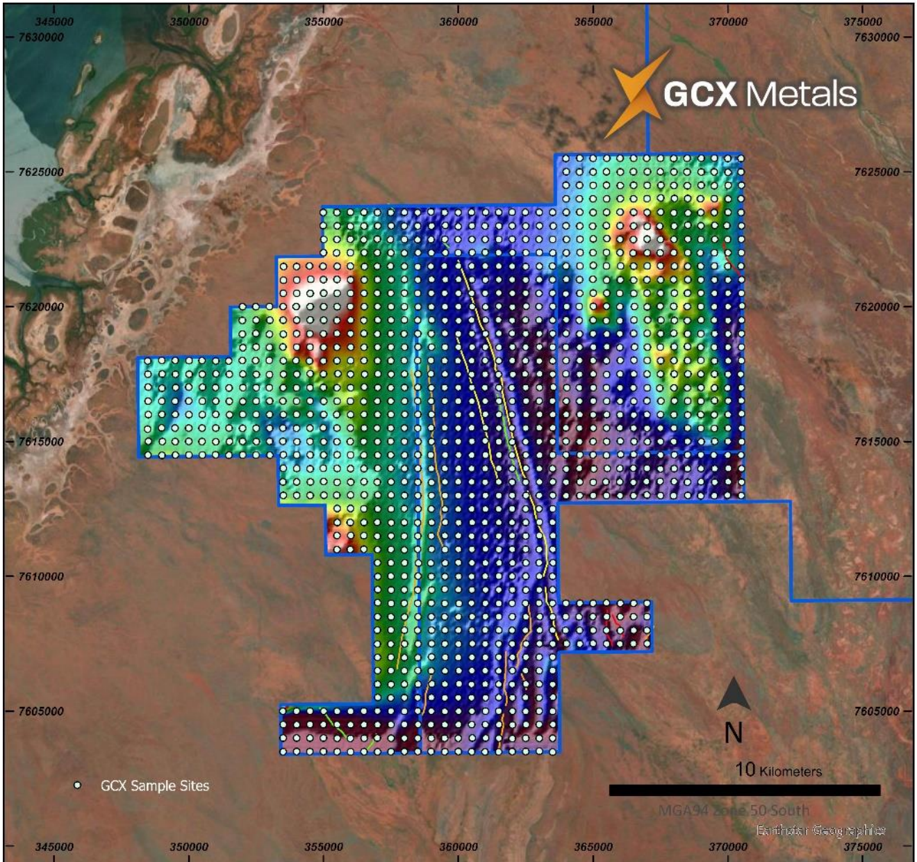
Figure 3: Soil Sample locations over AEM conductors and magnetics
