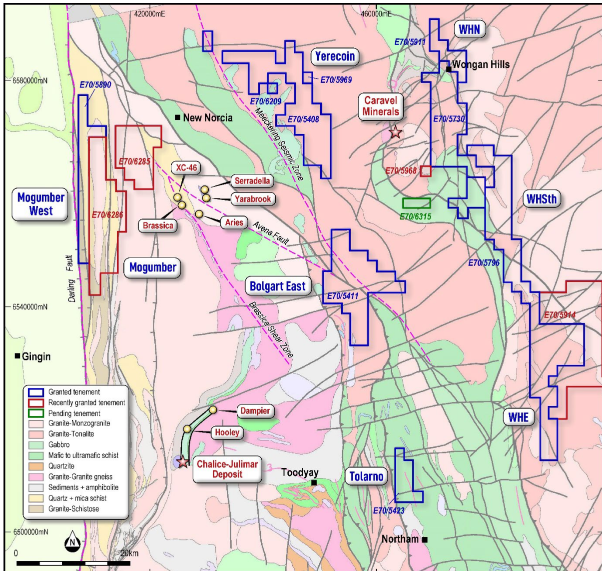
Figure 1: Julimar and WHS tenement position on 1:100 000 interpreted bedrock geology with local regional projects
