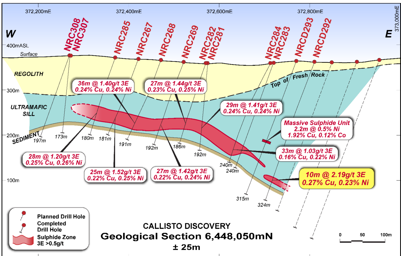
Figure 1 — Callisto geological interpretation section 6,448,050N with new mineralised zone in drill results from NRC292. Mineralisation is open to the east and north of NRC292.
