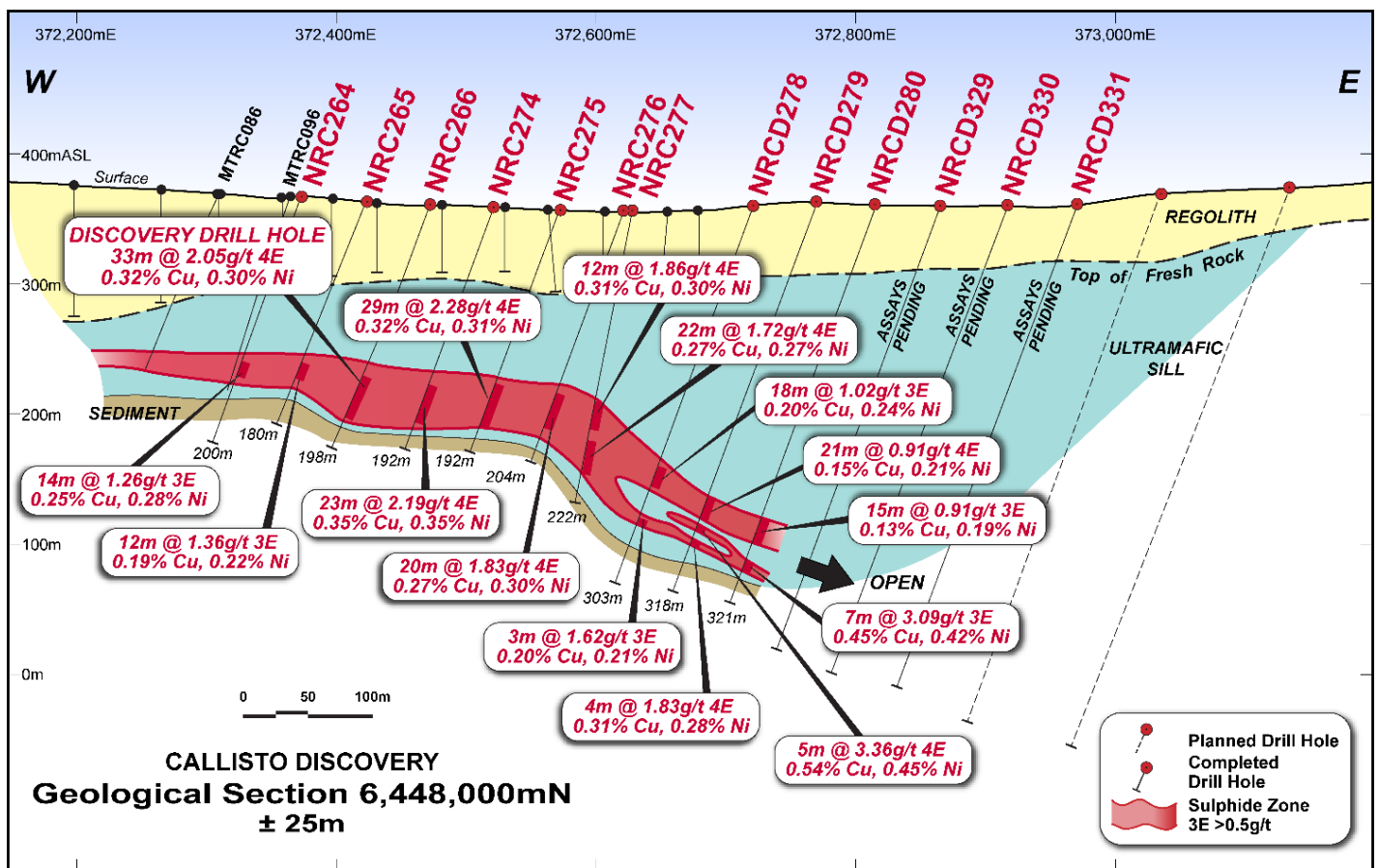
Figure 3 — Callisto geological interpretation section 6,448,000N with assays pending for drill holes NRCD329, NRCD330 and NRCD331. Mineralisation is open to the east.
