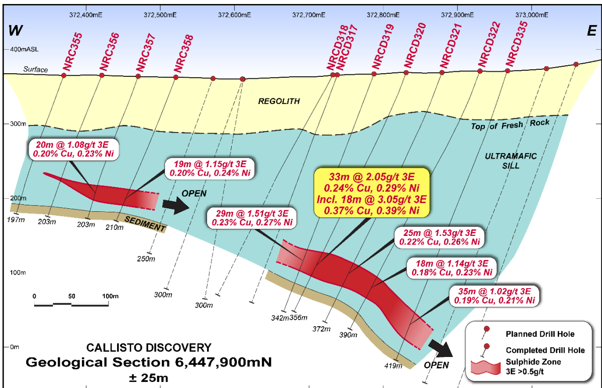
Figure 5 — Callisto geological interpretation section 6,447,900N with new assays for NRC321, NRC322 and NRC335 showing consistent mineralisation between drill holes. Mineralisation is open to the east and south.
