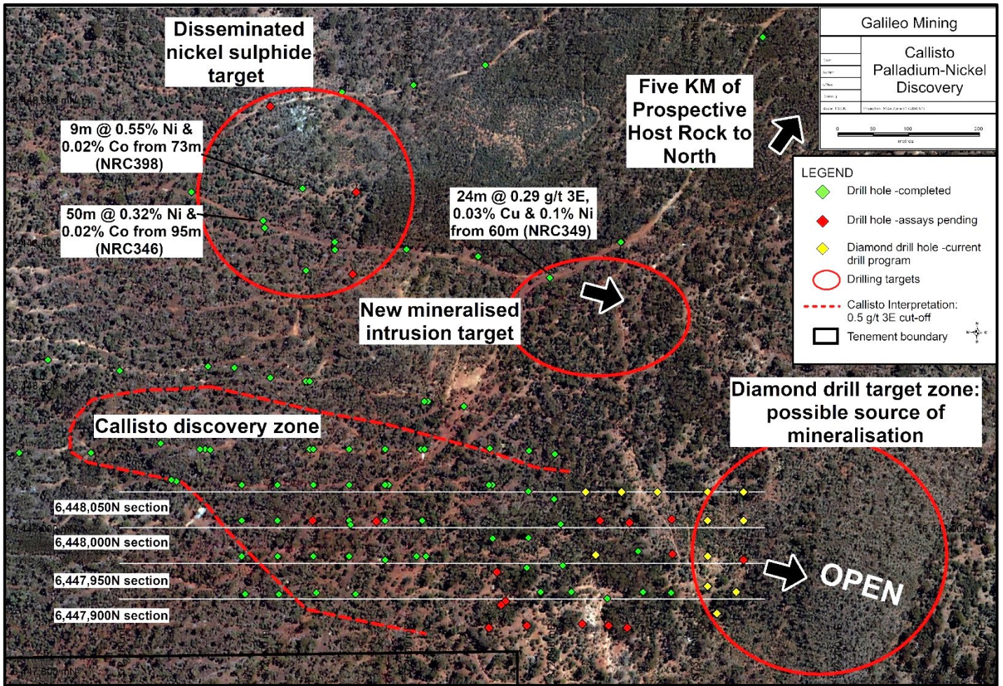
Figure 6 — Plan map of drilling at Callisto with priority drill target zones. Red dashed lines show the interpreted mineralised zone at 0.5 g/t 3E cut-off projected to surface. Source of mineralisation at Callisto is being targeted within the diamond drill zone as shown. Section lines are shown in Figures 1,3, 4 and 5.
