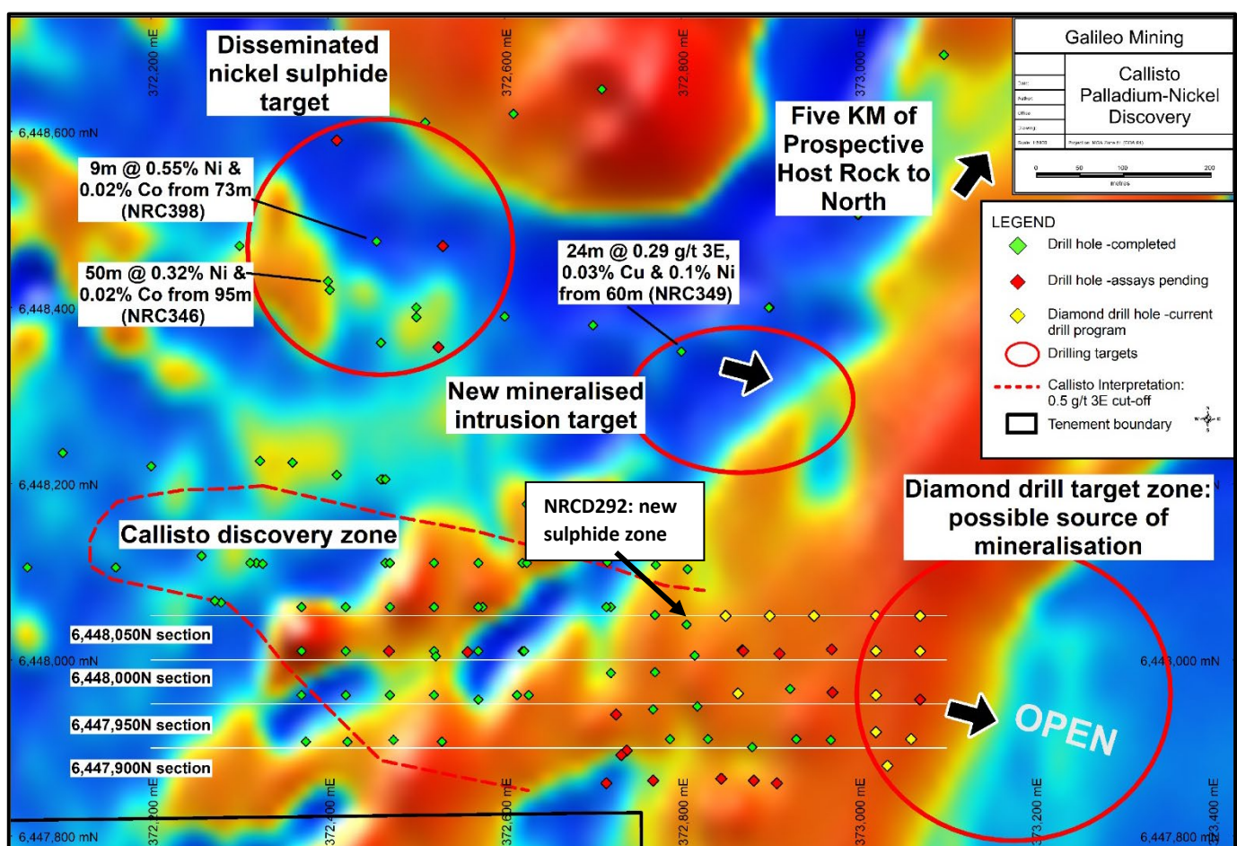
Figure 2 — Plan map of drilling at Callisto with priority drill target zones. Red dashed lines show the interpreted mineralised zone at 0.5 g/t 3E cut-off projected to surface. Source of mineralisation at Callisto is currently being targeted within diamond drill zone as shown. Section lines are shown in Figures 1,3, 4 and 5. Background magnetic image is TMI-1VD.
