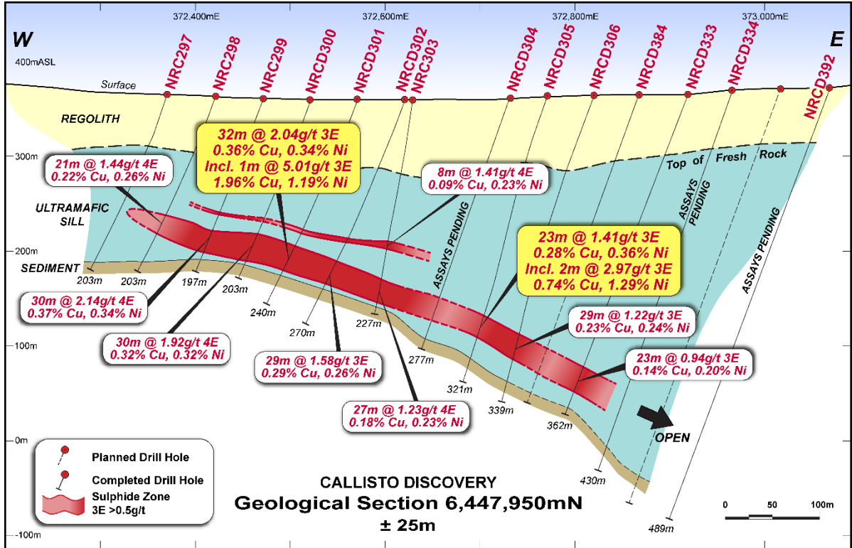
Figure 4 — Callisto geological interpretation section 6,447,950N with new assays for NRC302 showing consistent mineralisation between drill holes. Mineralisation is open to the east.
