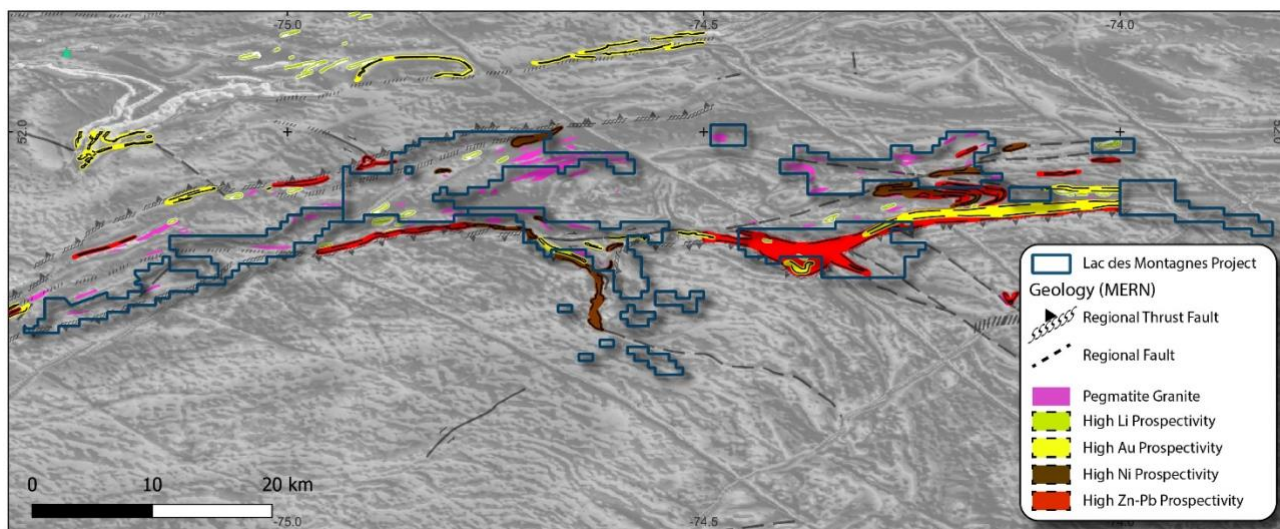
Figure 4: Results of prospectivity analysis (completed by MERN) identifying high-priority target areas for lithium, gold and base metal mineralisation.
