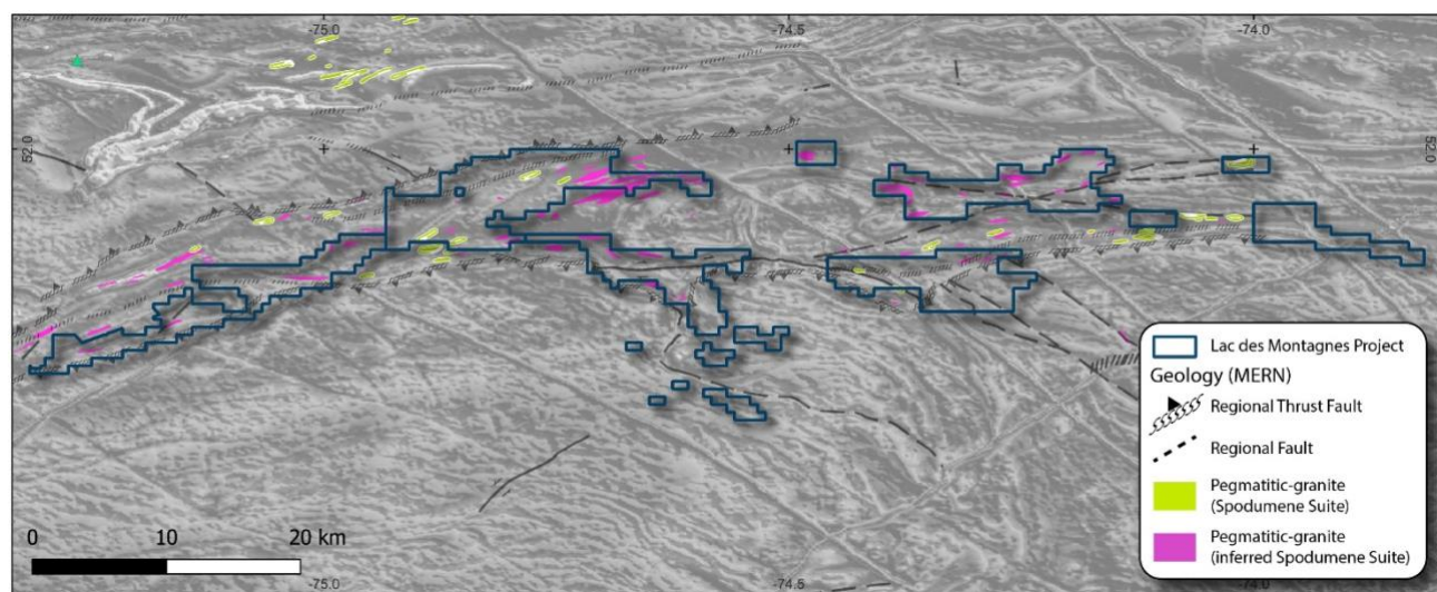
Figure 3: Distribution of pegmatitic granites (as mapped by MERN) over the Lac des Montagnes Project.
