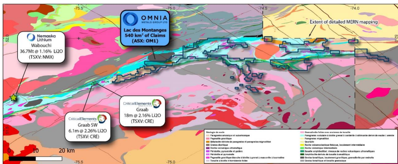
Figure 2: Geology of the Lac des Montagnes Project, Quebec, Canada.
