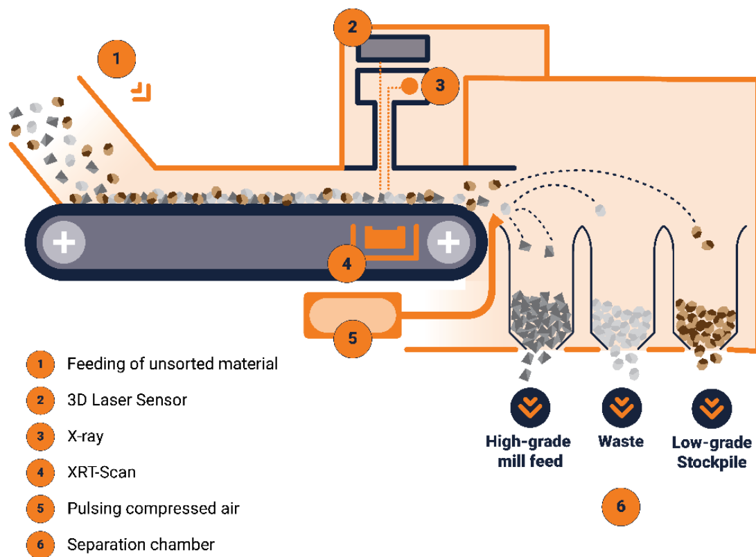
Figure 1: Steinert KSS XT CLI Ore Sorter
