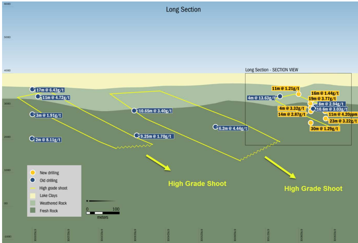
Figure 2b: Long Section of Fortitude North with new drilling (see inset next image 2c)
