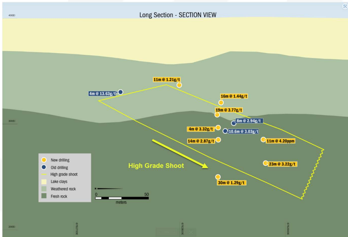
Figure 2c: Long Section of Fortitude North high grade shoot (refer Figure 2b)
