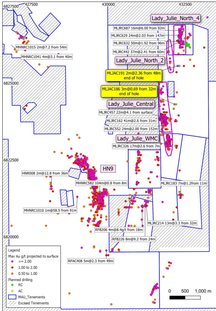
Figure 2 Gold intersection overview covering the HN5, HN6, HN9 and adjacent Lady Julie Projects showing some highlighted intersections (white label). Significant historical and Magnetic intercepts (maximum Au projected to surface) and highlighted AC results in yellow along the Chatterbox shear extending south from the Lady Julie North 4 Deposit.
