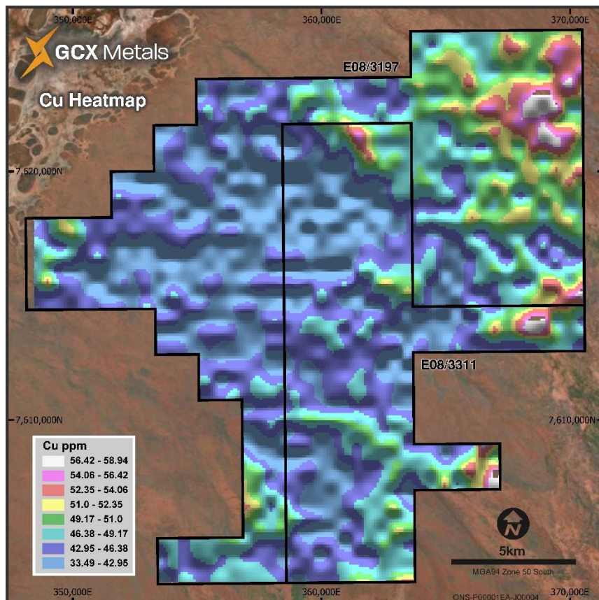
Figure 3: Copper Soil Sample Anomalies
