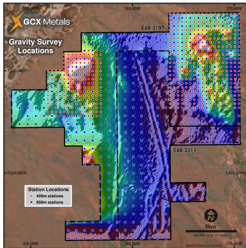
Figure 5: Planned Gravity Survey Stations (over TMI magnetic image)
