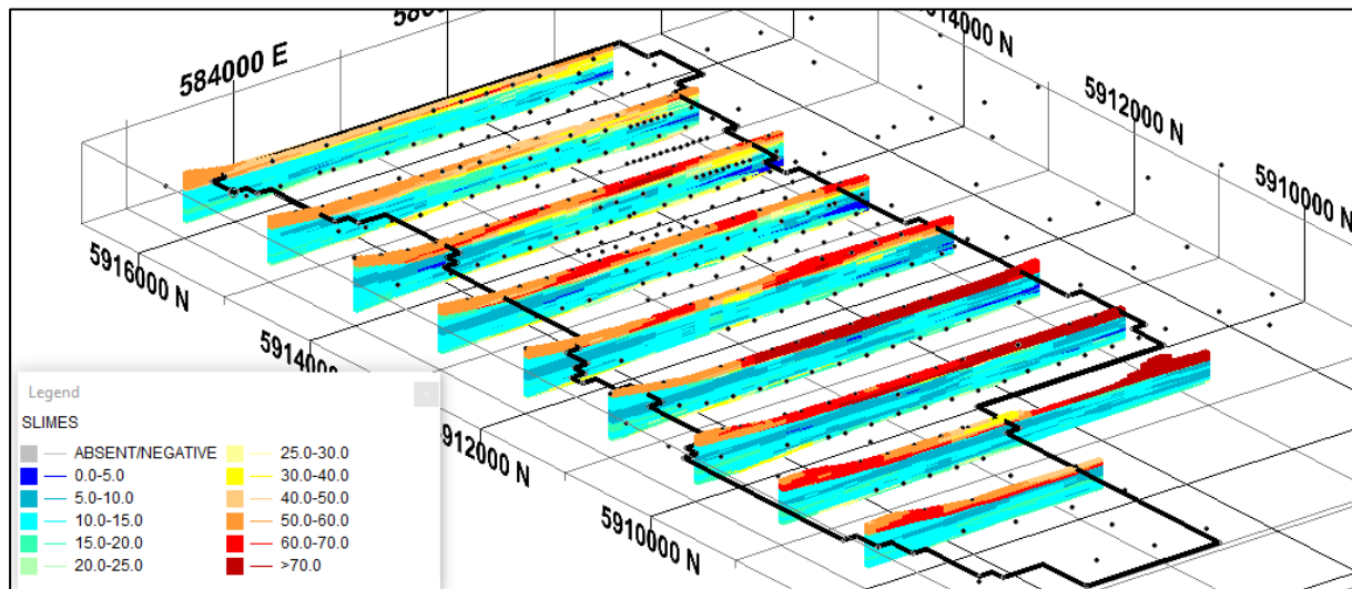
Figure 8: WIM100 deposit block model slices showing Slimes grade, (20x vertical exaggeration).
