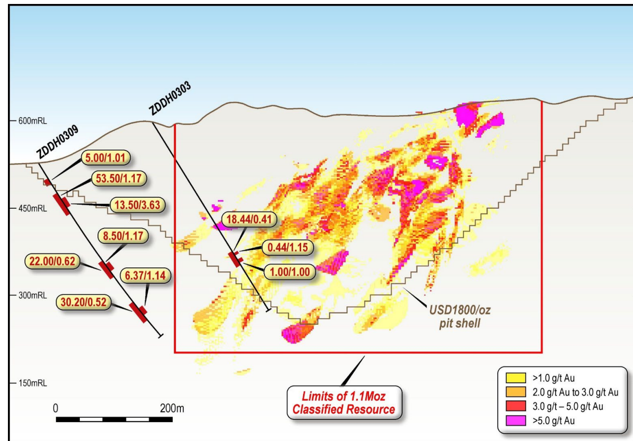
Drill Section looking west with MRE block model. Block model coloured to gold grade. Hole ZDDH0309 2 is drilled approximately 200m outside of the MRE limit. Window +/-25m, datum PSAD56 19S.
