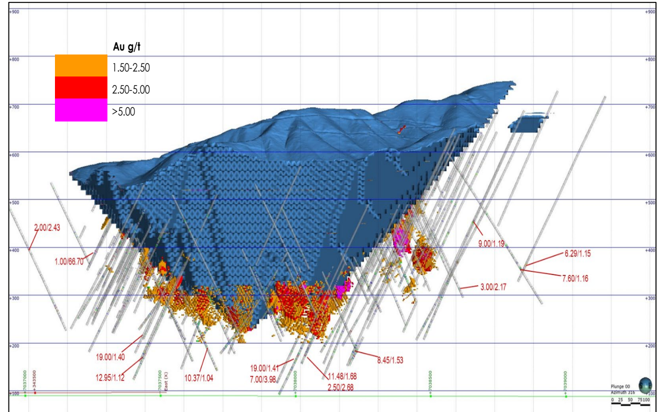
3D view looking northwest of the Ternera MRE block model, US$1,800pit shell. Multiple high-grade zones below pit for potential underground mining. Drilling with selected drill highlights (downhole width/Au g/t) showing extensions requiring further drilling for resource classification - 100m grid.
