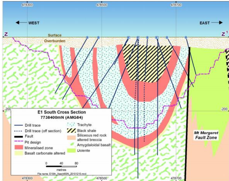
Figure 3 - Cross Section of E1 South Pit
