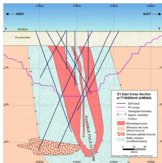
Figure 4 - Cross Section of E1 East Pit
