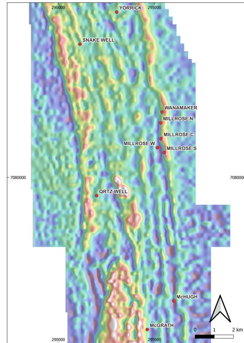
Gravity image overlay by locations of the McGrath, Quartz Well and Snake Well prospects along the eastern margin of the Baxter's Greenstone Block (gravity high).
