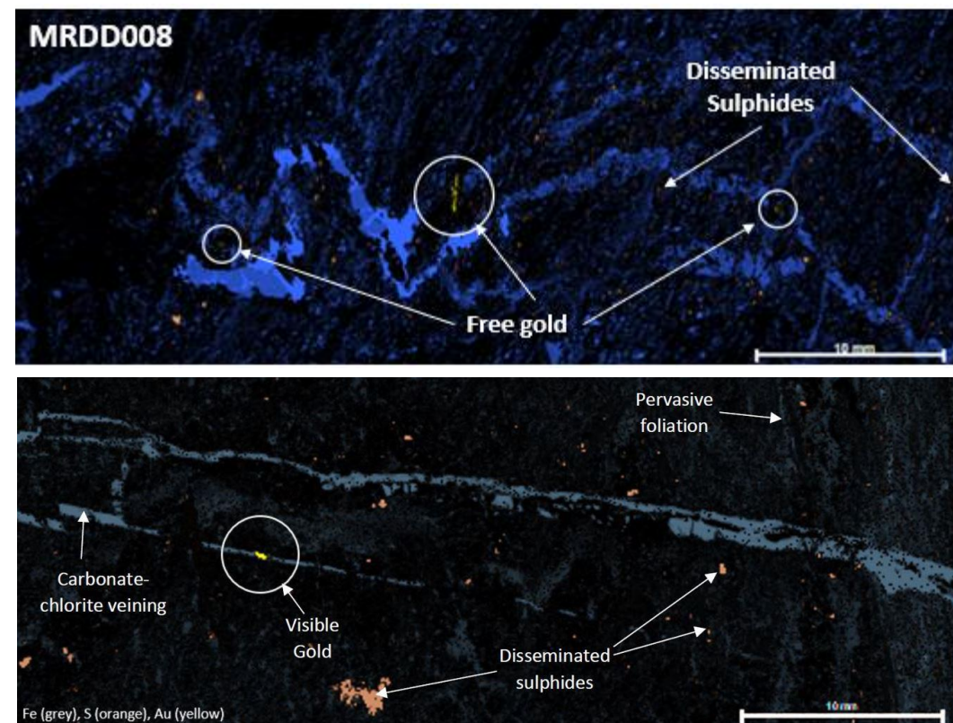
Top: Micro XRF image showing free gold associated with sheared veinlets in MRDD008. Bottom: Micro XRF image of free gold in D3 vein.
