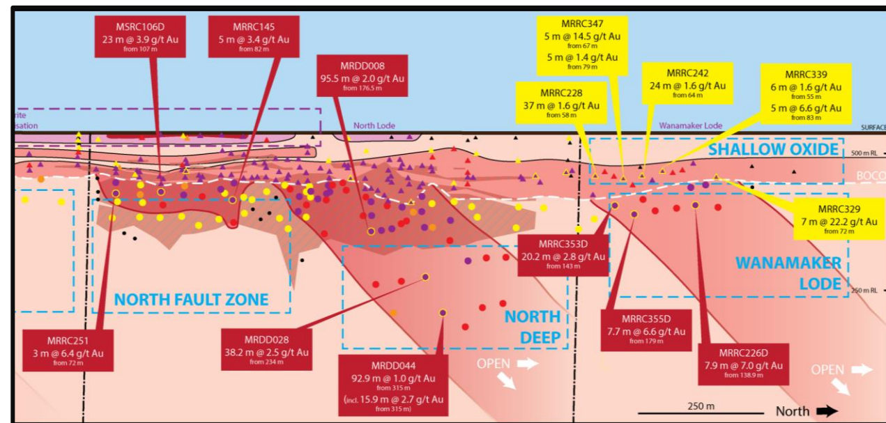
Long section of Millrose North and Wanamaker.
