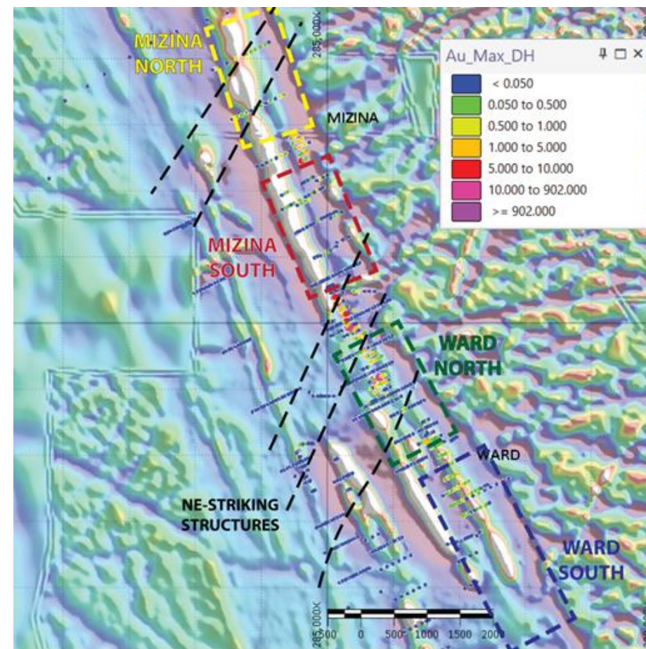
Mizina-Ward drilling coded by maximum downhole gold. NE-striking regional structures shown by black dashed lines, and target zones for exploration outlined.
