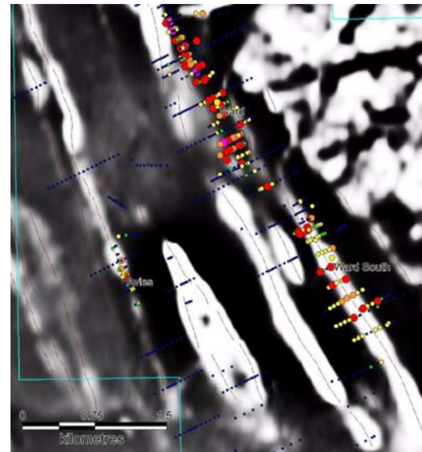
Avies location and drilling coded by maximum downhole Au.
