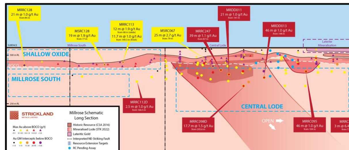
Long section of Millrose Central and South.
