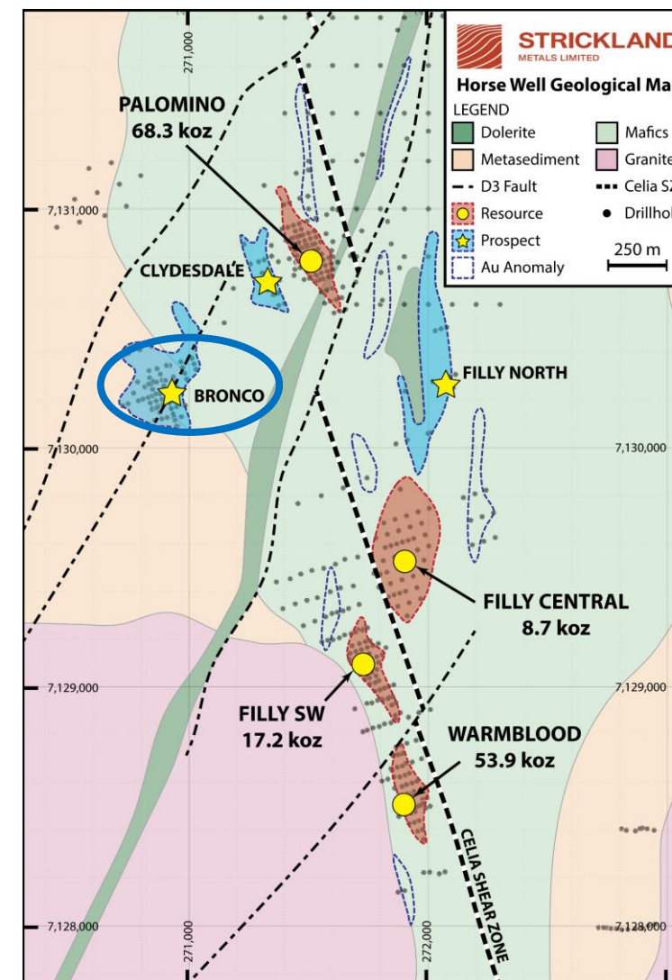
Horse Well map highlighting advanced prospects (blue) and resources (red)
