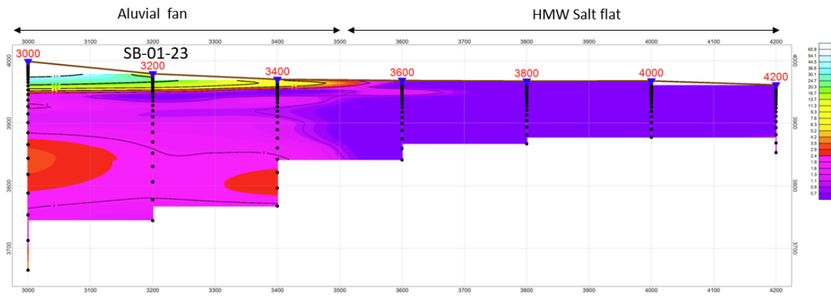
Figure 4. TEM section 1880.
