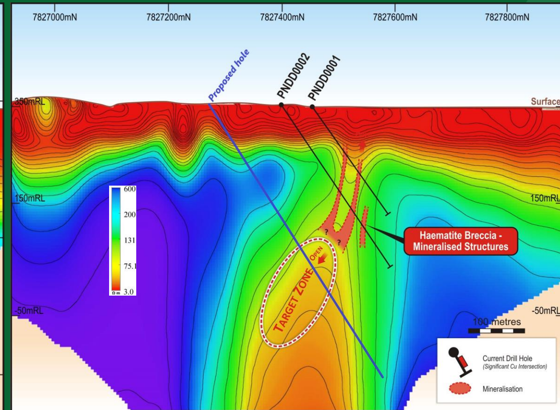
Perseverance North cross-section 447,700mE 7
