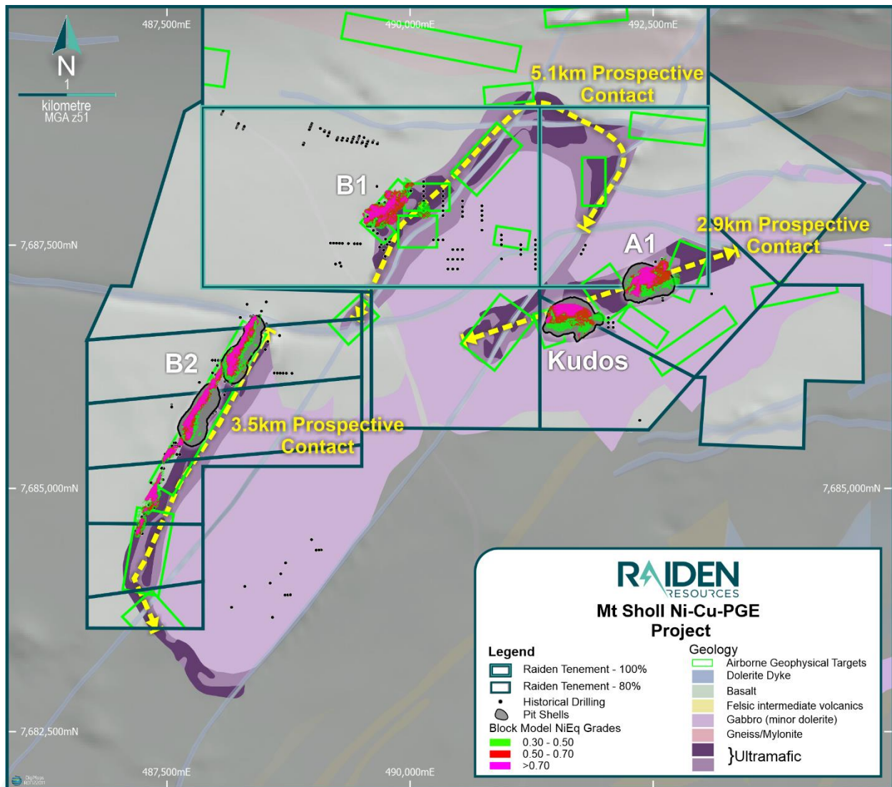
Figure 11 : Mt Sholl 2023 Exploration Target Areas with prospective contact zones overlain on the 2021 Exploration Target
