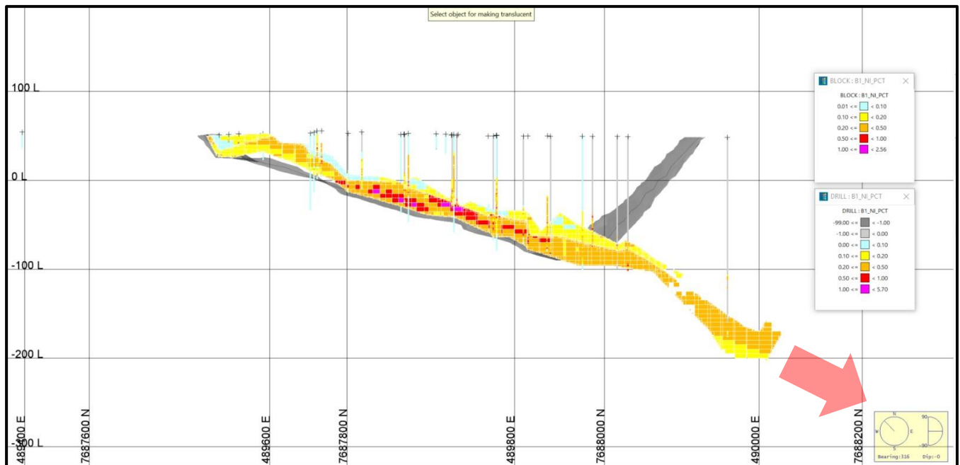
Figure 8: Long-section B1 pit (at 0.35%Ni_Eq cut-off) and mineralisation – view to the northwest
