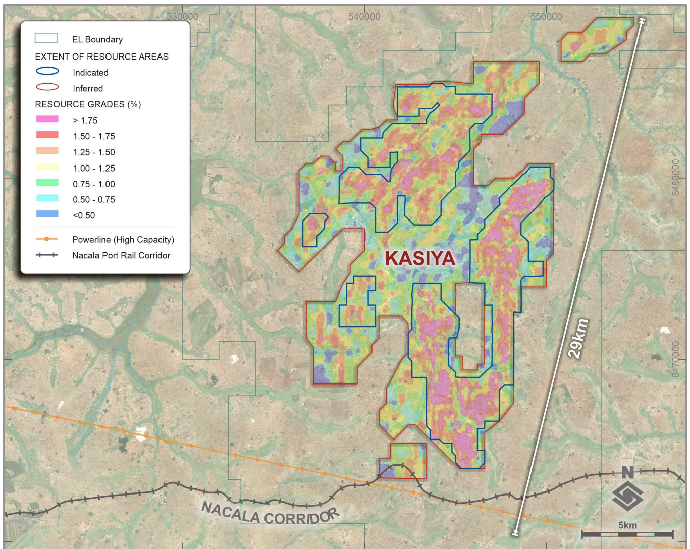
Figure 2: Kasiya map showing rutile grades of the upper blocks of the MRE block model
