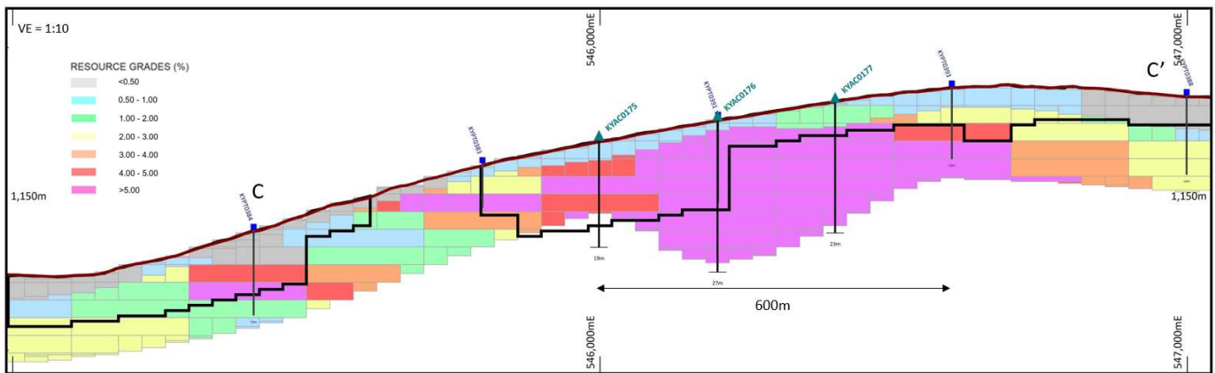
Figure 4: C-C' cross-section from the southern part of the MRE block model in a higher-grade graphite zone showing colouring by graphite grade (TGC) with previous ESS pit shapes also shown. Refer Figure 5.
