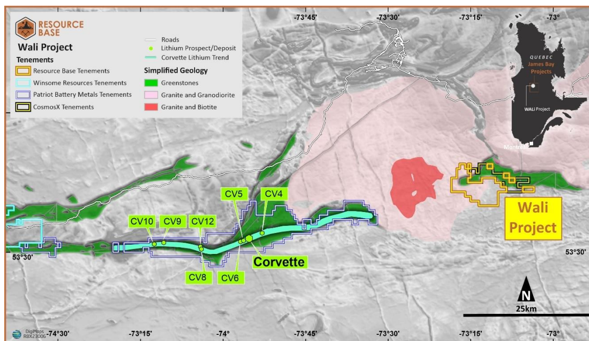
Figure 1: Location of the Wali Project, James Bay Lithium Region over simplified geology
