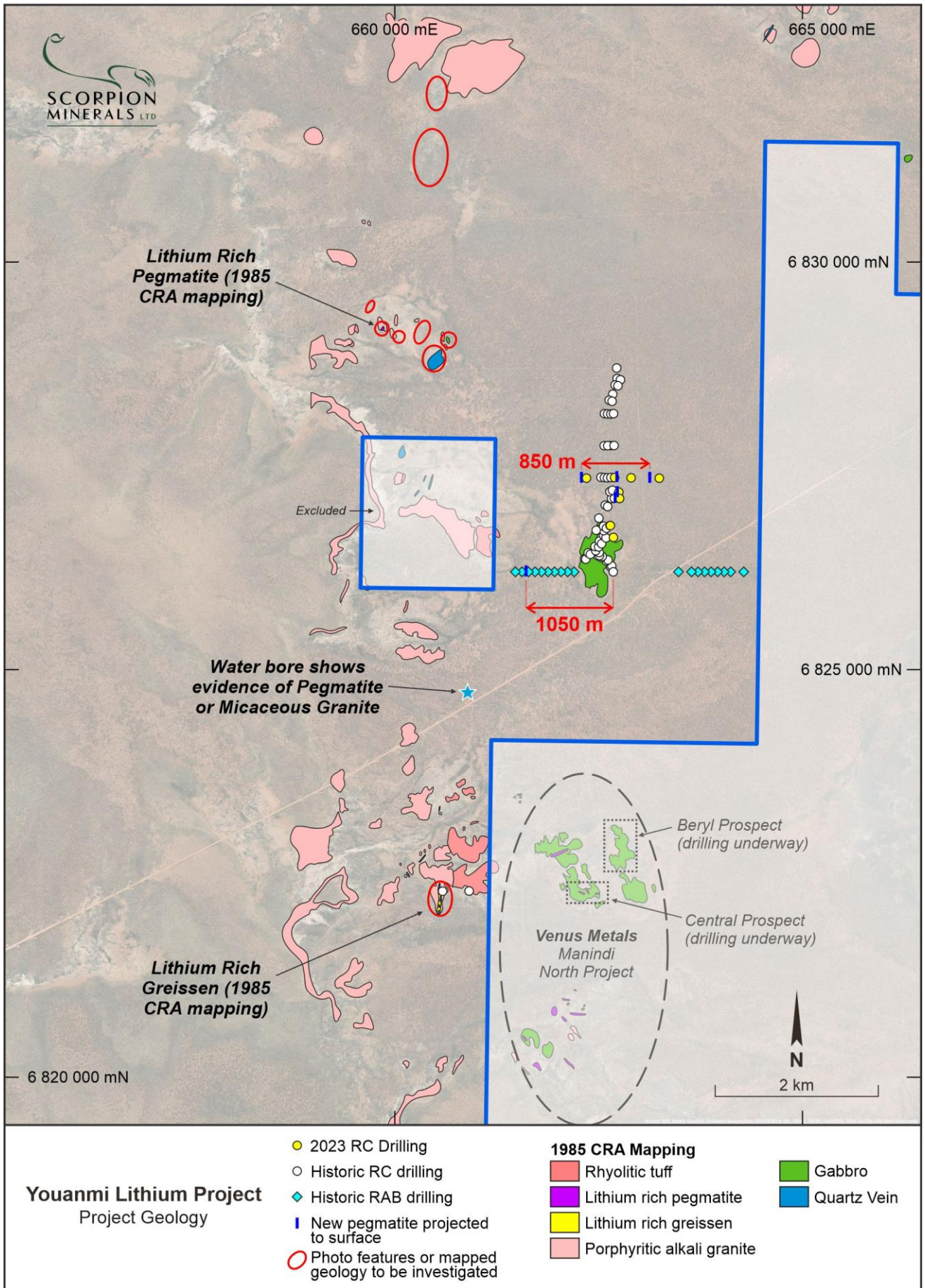
Figure 3: Regional Geology
