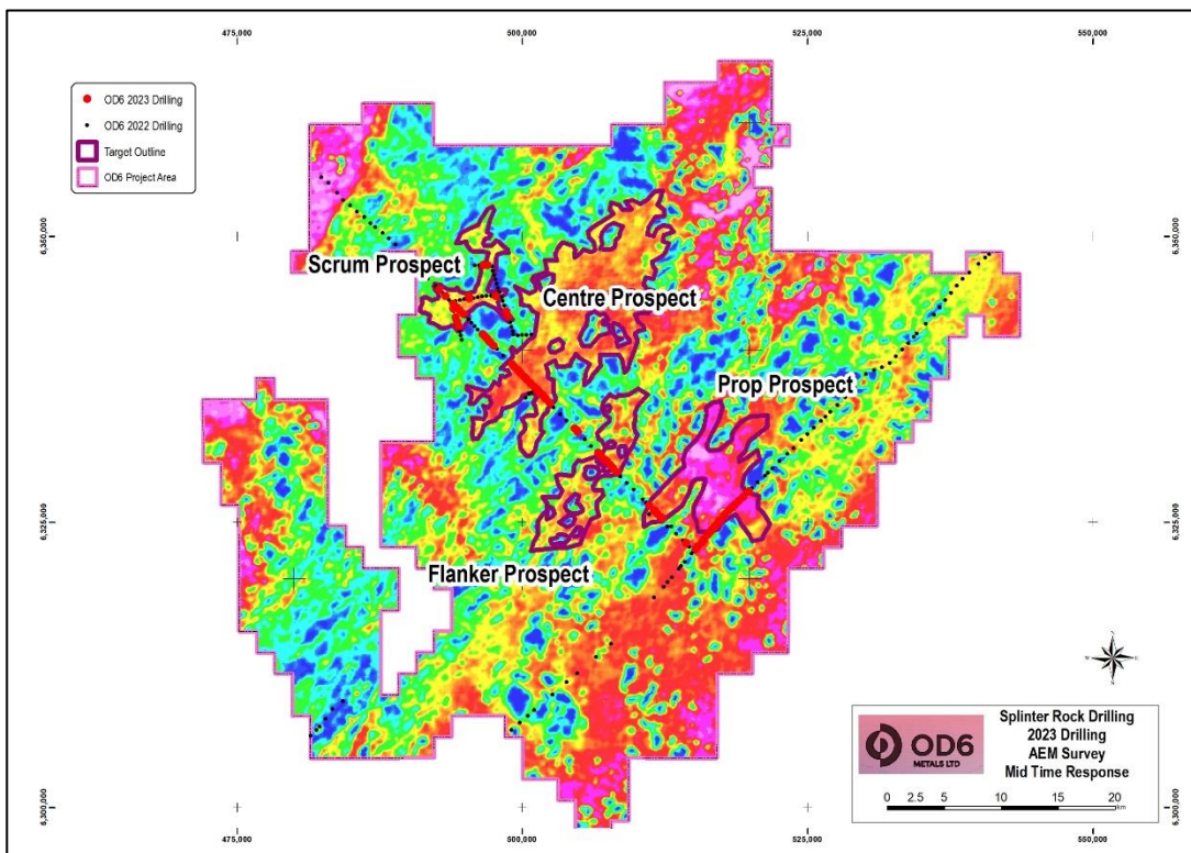
Figure 6: AEM Mid time electromagnetic conductivity model of Splinter Rock Project with drilling locations. Yellow, red, pink areas interpreted to indicated thicker clay zones, with blue areas the granites). Refer to ASX Announcement, 15 December 2022 )
