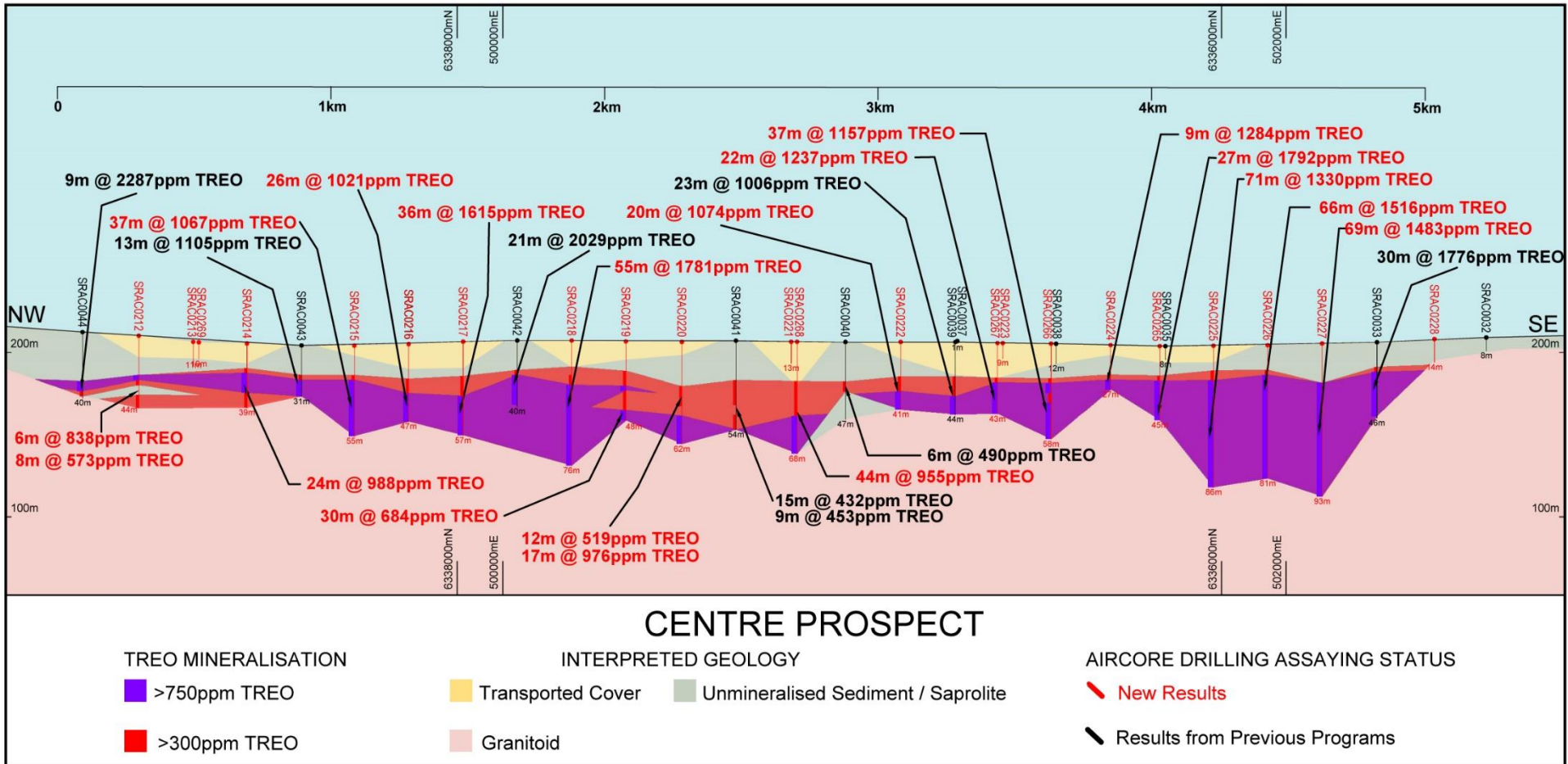
Figure 1: Centre Prospect Cross Section (vertical exaggeration x6)
