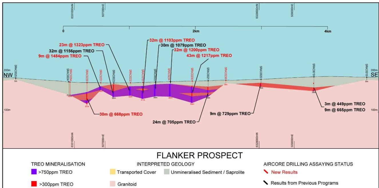
Figure 4: Flanker Prospect Cross Section (vertical exaggeration x6)
