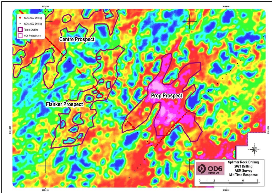
Figure 8: AEM Mid time electromagnetic conductivity model of Flanker and Prop Prospects with infill drilling locations shown in red. (Yellow, red, pink areas interpreted to indicated thicker clay zones, with blue areas the granites).
