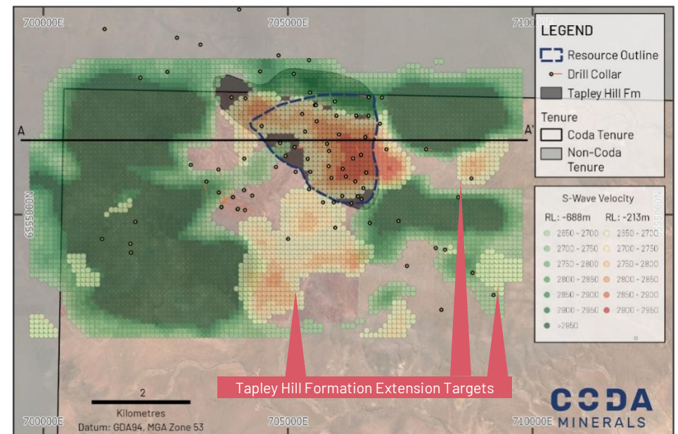
Figure 5 (Right) Plan view showing the ANT velocity model** at -213m RL (Emmie Bluff Copper-Cobalt Mineral Resource depth, red colours) and at -688m RL (Emmie IOCG mineralised depths (green colours). Note the negative correlation between the (interpreted) Tapley Hill Formation shale and the high velocity signatures in the basement, suggesting topographic control of the shale deposition.
