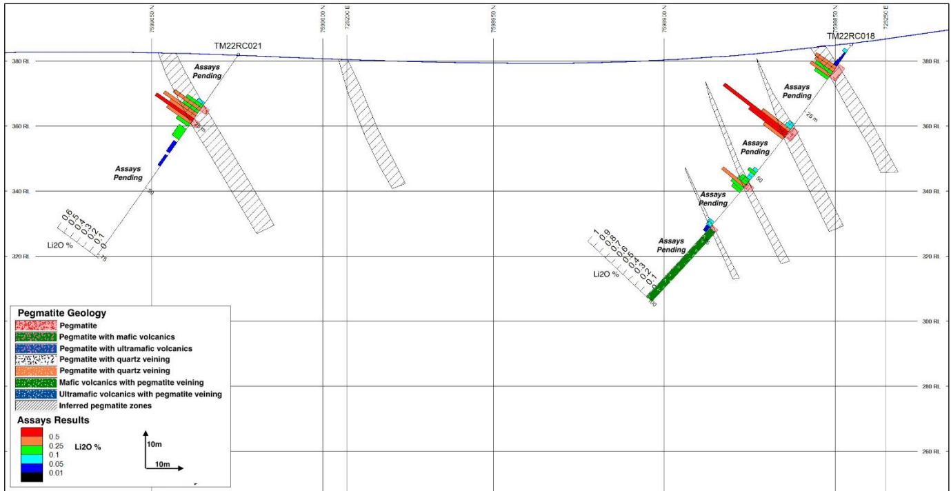
Figure 4. Cross-section 2, Naughton's area.
