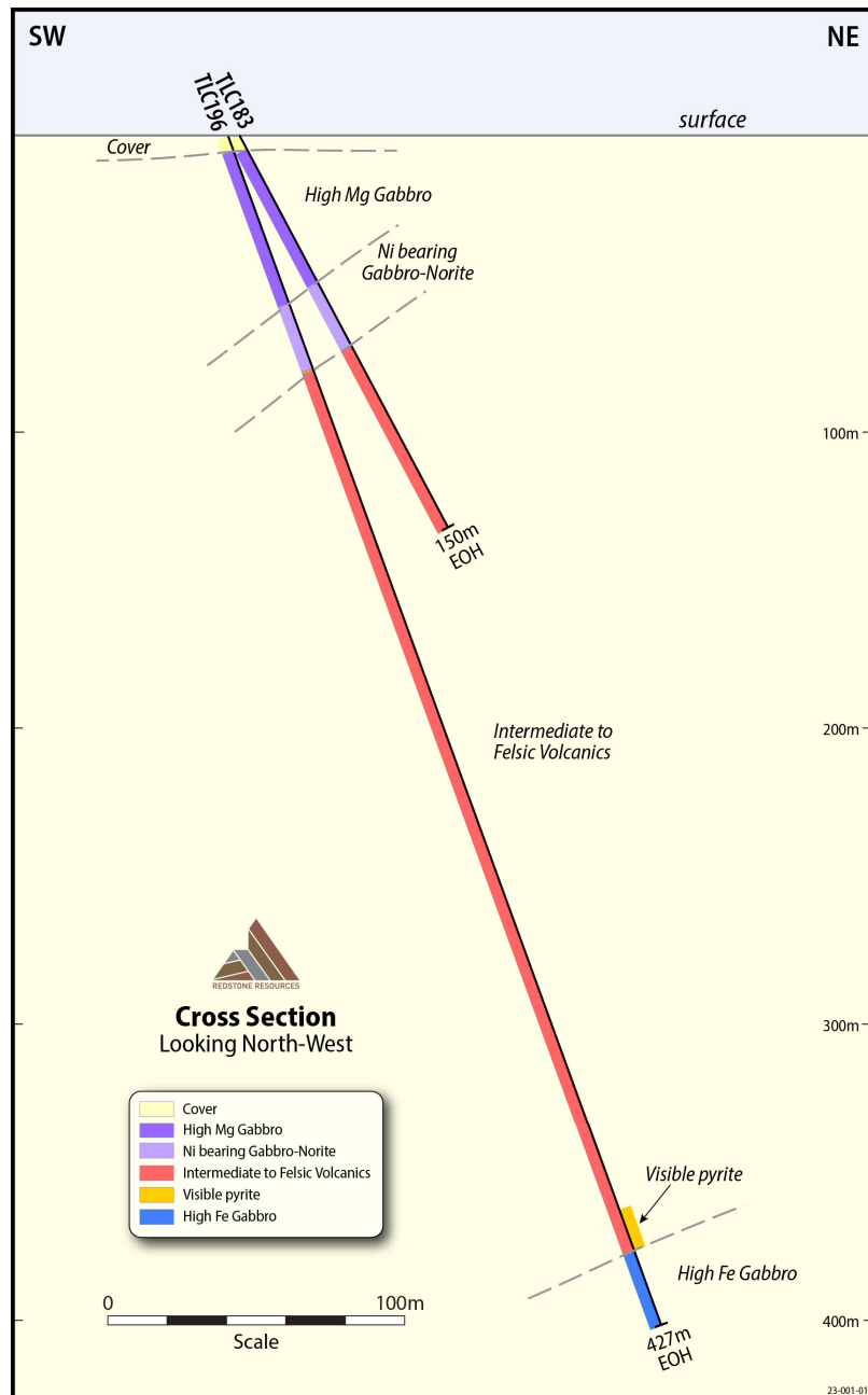
Figure 2: Geological cross-section looking NW through RC drill holes TLC183 and TLC196 showing the intersection of the high Mg-Ni-Cr layered mafic-ultramafic intrusion. See text for further details.
