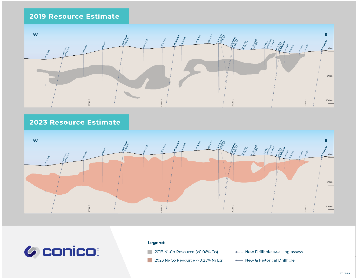
Figure 3: Mt Thirsty Main geological cross-sections showing near-surface resource additions. 2.5x vertical exaggeration. 644770N
