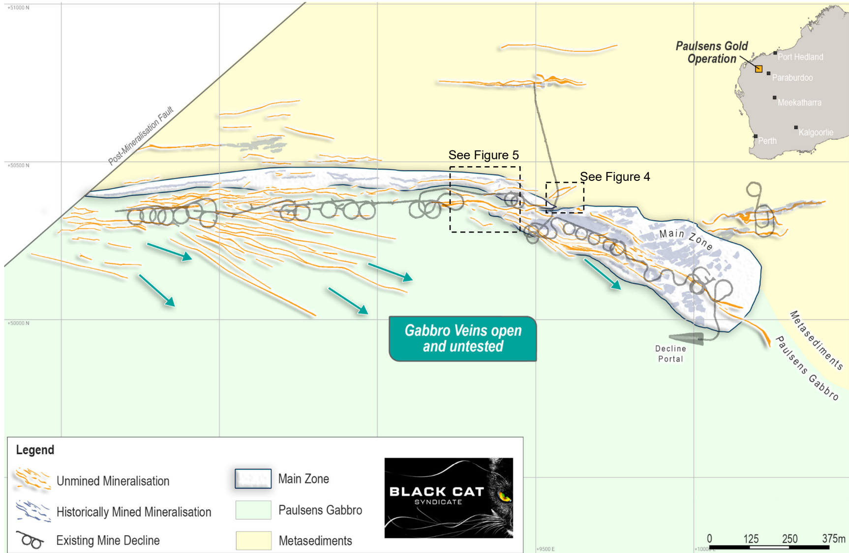
Figure 3: Plan view showing the location of the unmined, high-grade Gabbro Veins, the mined and unmined portions of the Main Zone, which produced ~1,000oz per vertical metre from narrow lodes within the Main Zone. Recent drilling has focussed on near-surface targets. The 7km long dewatered decline provides easy access to the recently identified mineralisation. View is in mine grid.
