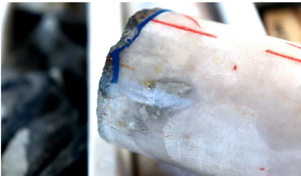
Figure 1: Visible gold in PGRD23101. This interval returned 0.26m @ 197.00g/t Au from 50.24m.
