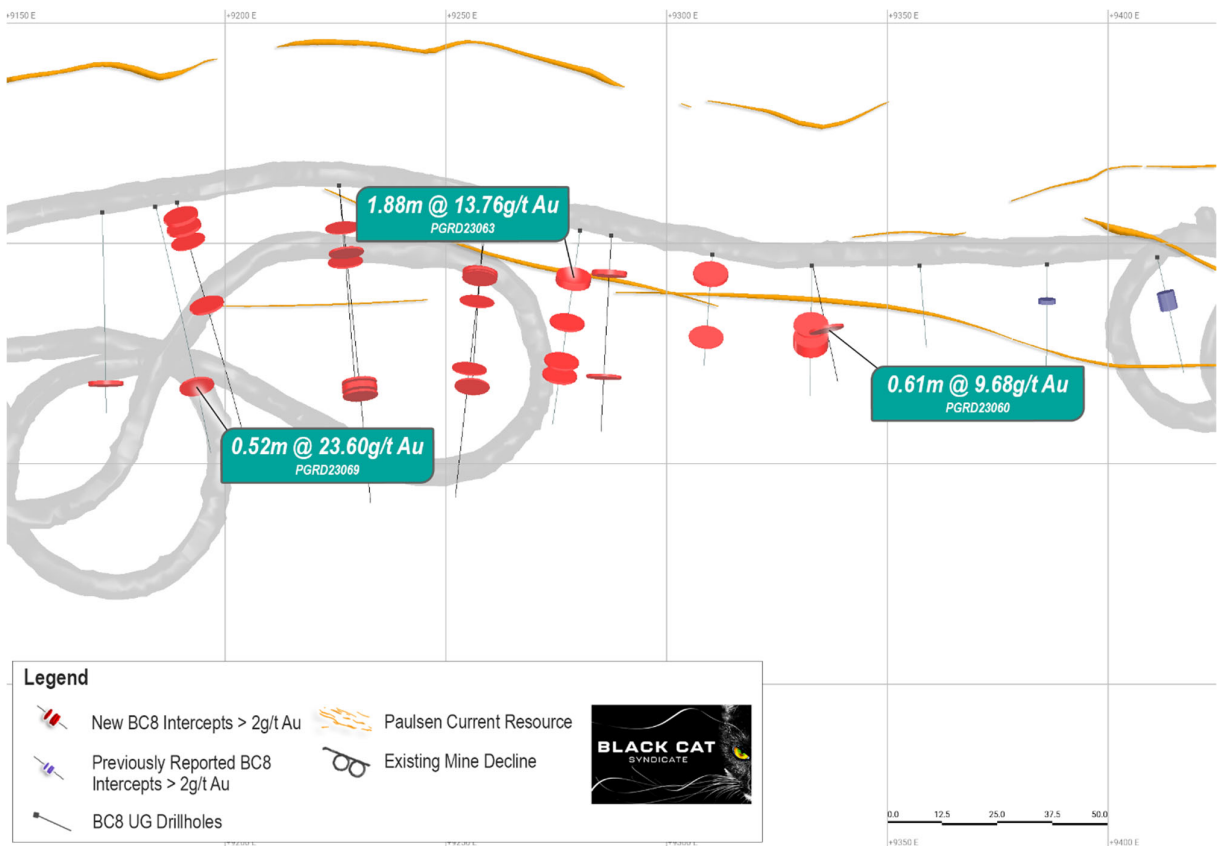
Figure 5: Drilling results in Main Zone located in the middle part of the mine showing numerous mineralised veins with high-grade intercepts highlighted (see Figure 3)
