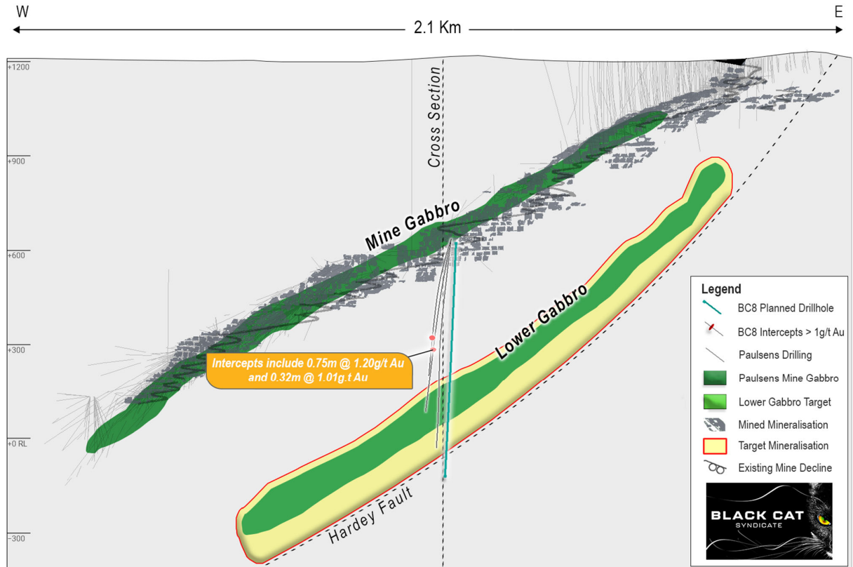
Figure 6: Schematic long-section looking north showing the Paulsens Repeat target below existing workings.
