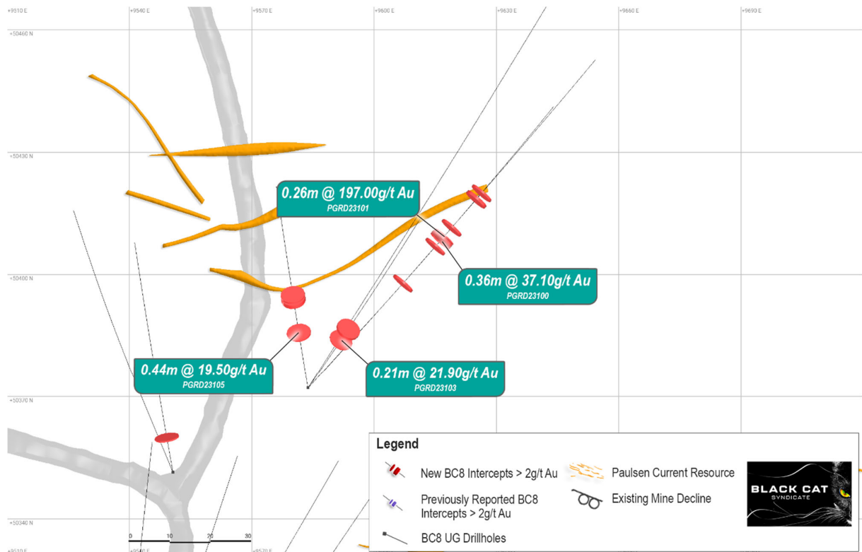
Figure 4: Drilling results in the middle part of the mine showing numerous mineralised veins with high-grade intercepts highlighted (see Figure 3)
