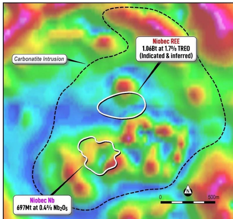
Figure 1. Reprocessed ground magnetics at Schryburt showing new targets (above) and airborne magnetics at Niobec 1 showing the location of the REE resource in a magnetic low (below)
