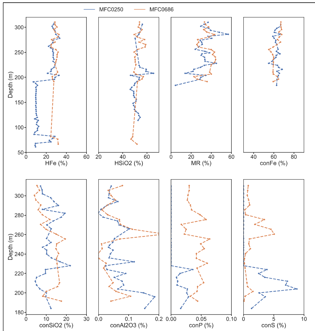
Figure 4-7: Historical RC (blue) and new RC (orange) twin pair comparison
