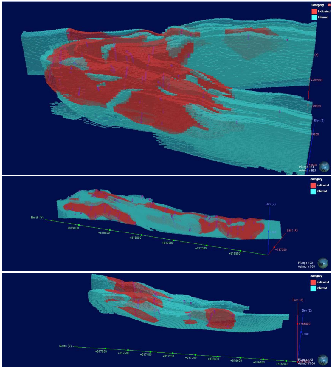
Figure 5-28: Mineral Resource classification for MF1 (top), MF2 (middle), and MF6 (bottom)
