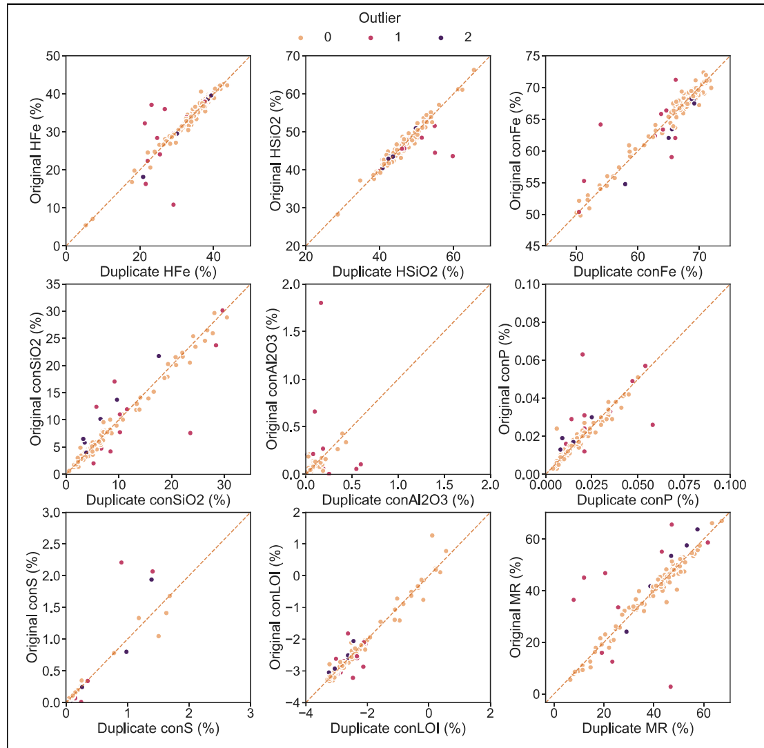
Figure 4-3: Performance of duplicate samples
