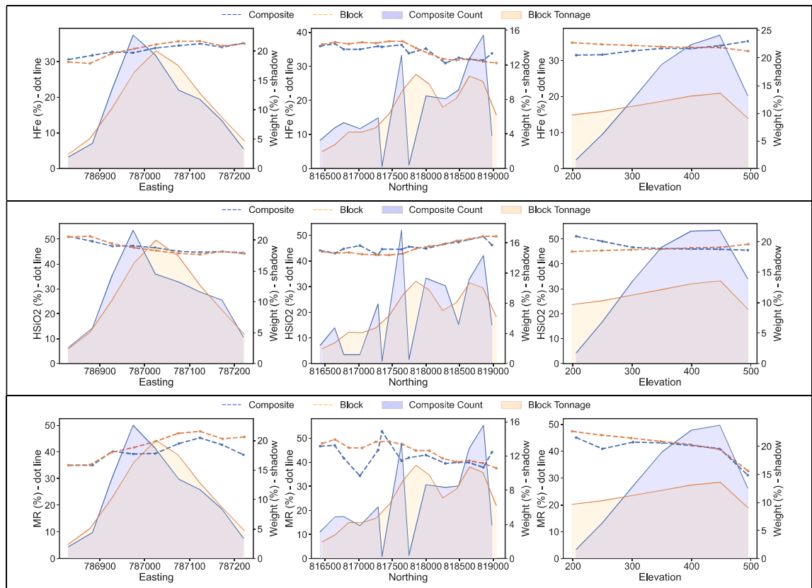
Figure 5-26: Swath plots for MF2
