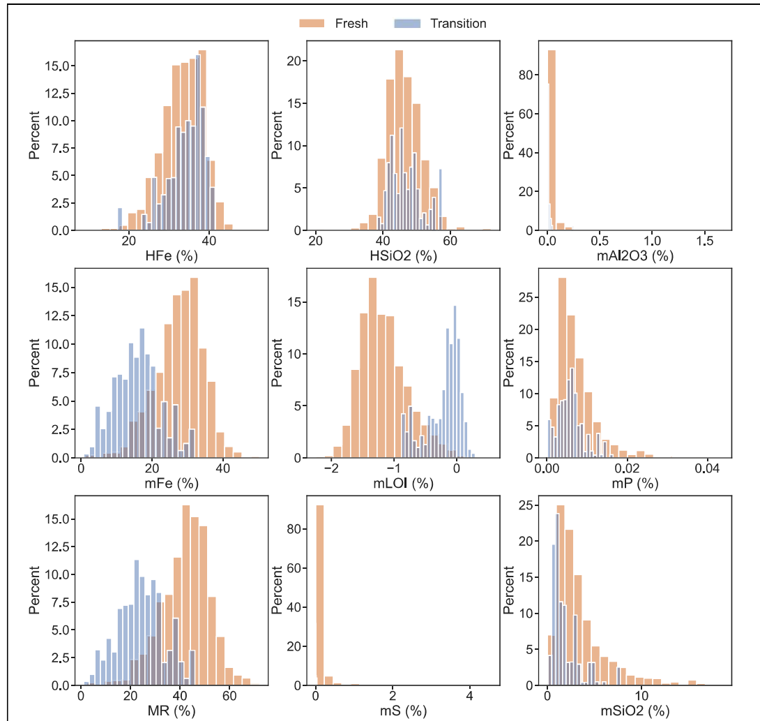
Figure 5-7: Histograms for elements in MF2
