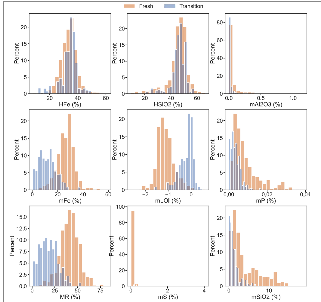
Figure 5-6: Histograms for elements in MF1
