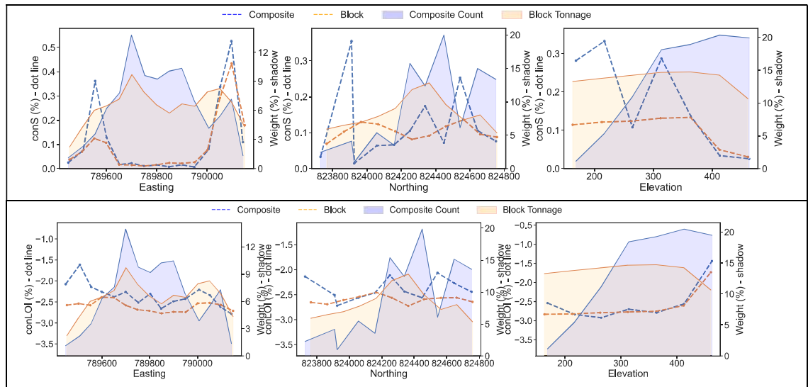
Figure 5-26: Swath plots for MF2
