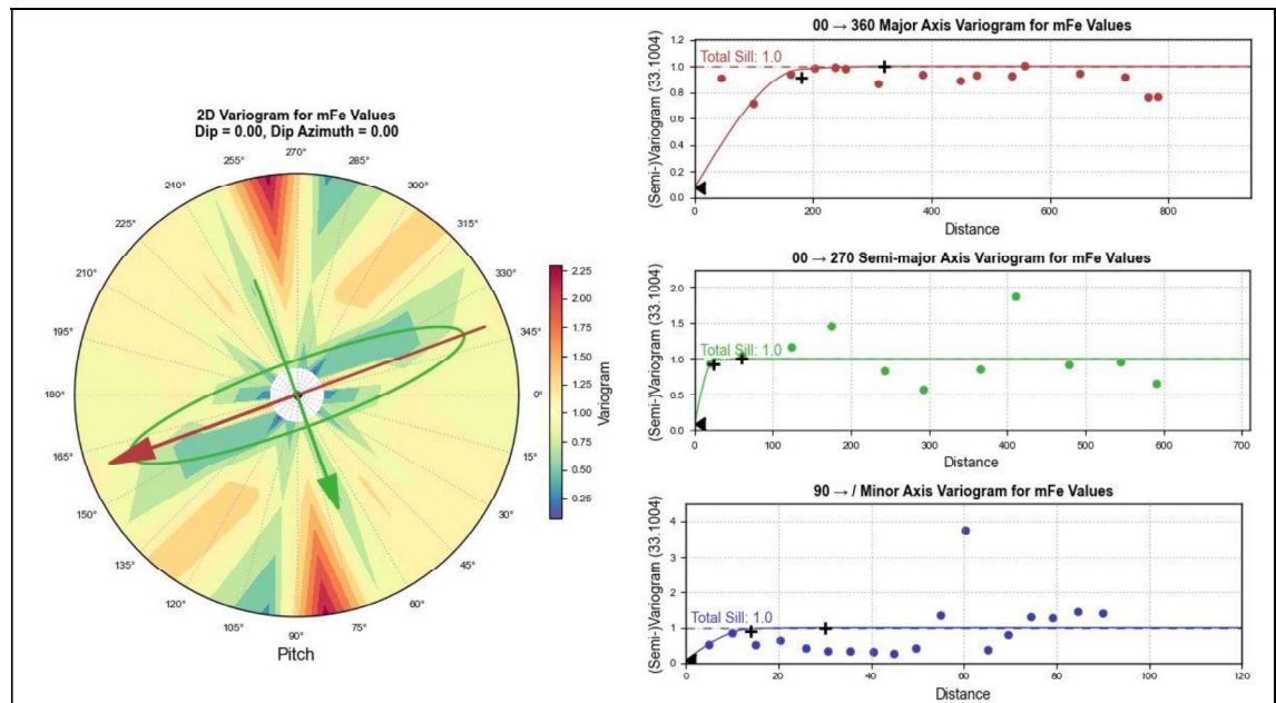
Figure 5-12: Variogram model for mFe in MF1 transition domain
