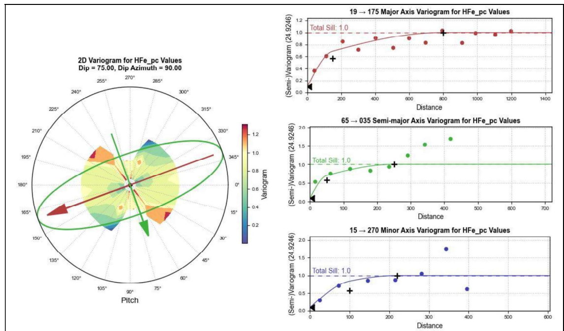
Figure 5-13: Variogram model for HFe in MF2 fresh domain
