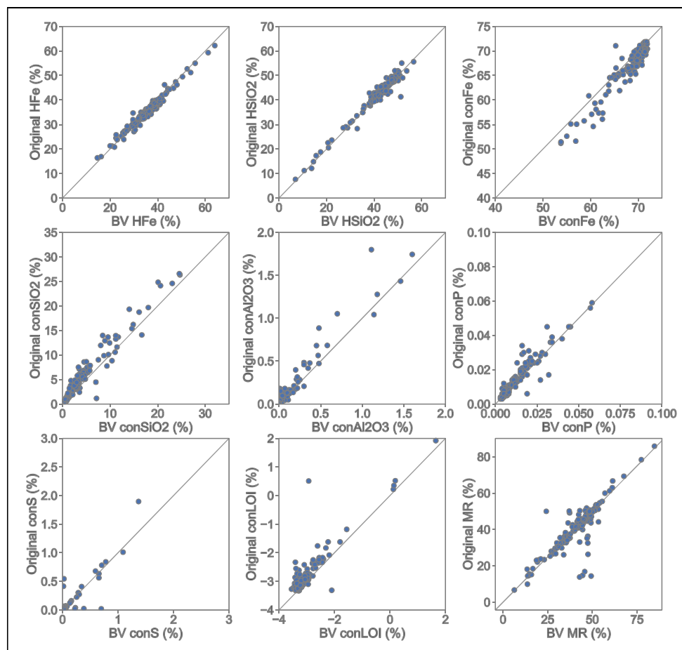
Figure 4-8: Performance of Independent laboratory check
