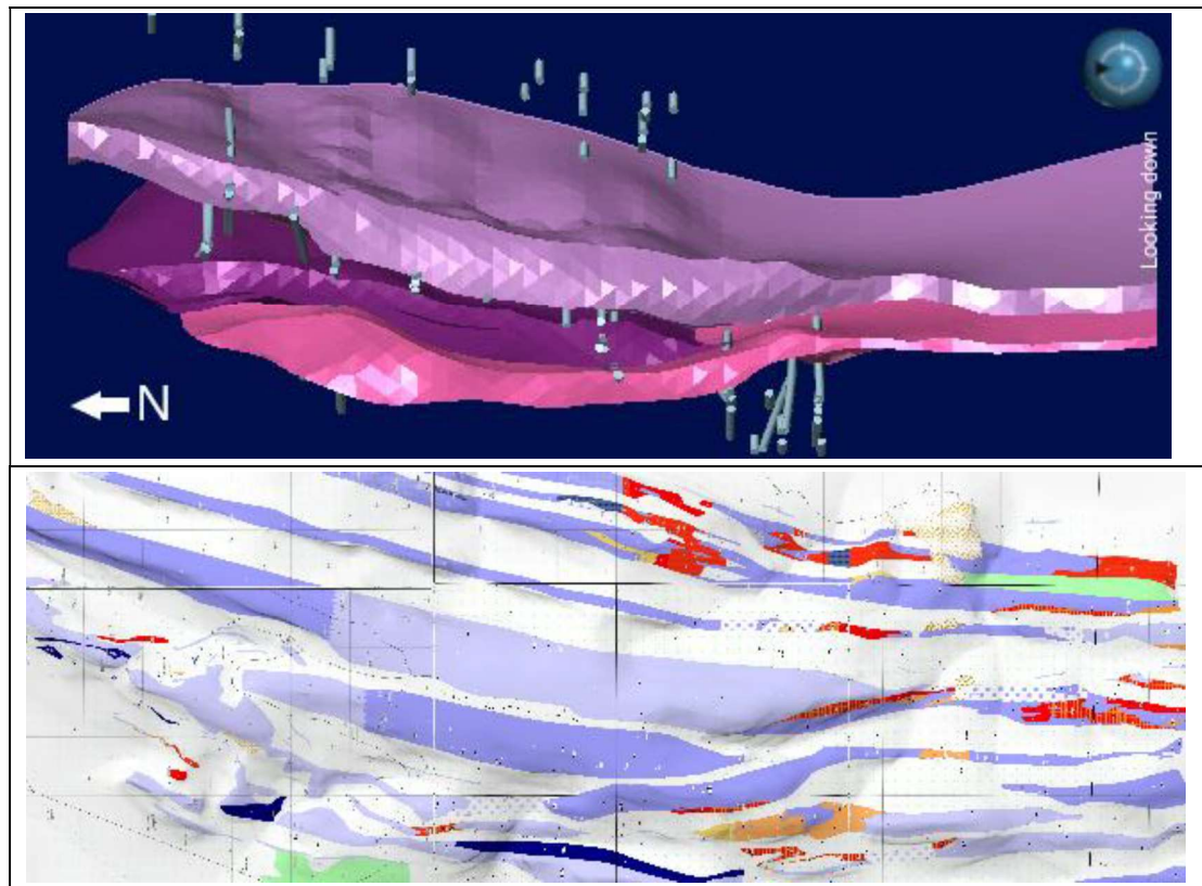
Figure 5-3: Top view of MF6 BIF model (above) and local geological map (below)
