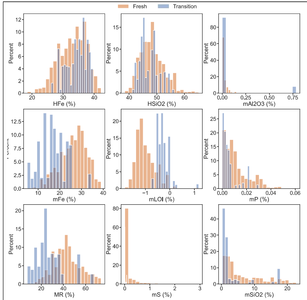
Figure 5-8: Histograms for elements in MF6
