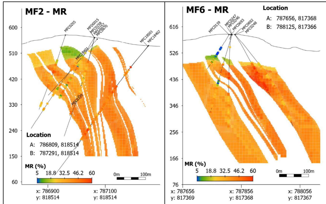
Figure 5-23: Cross section of MF2 and MF6 showing MR in blocks versus drill holes
