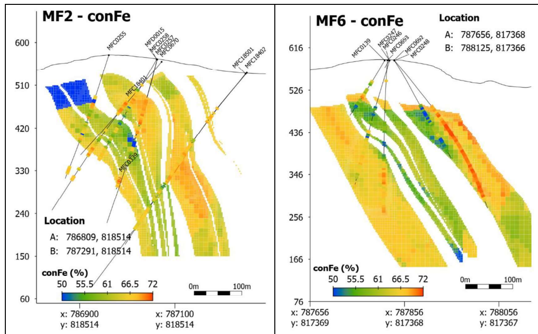
Figure 5-24: Cross section of MF2 and MF6 showing conFe in blocks versus drill holes
