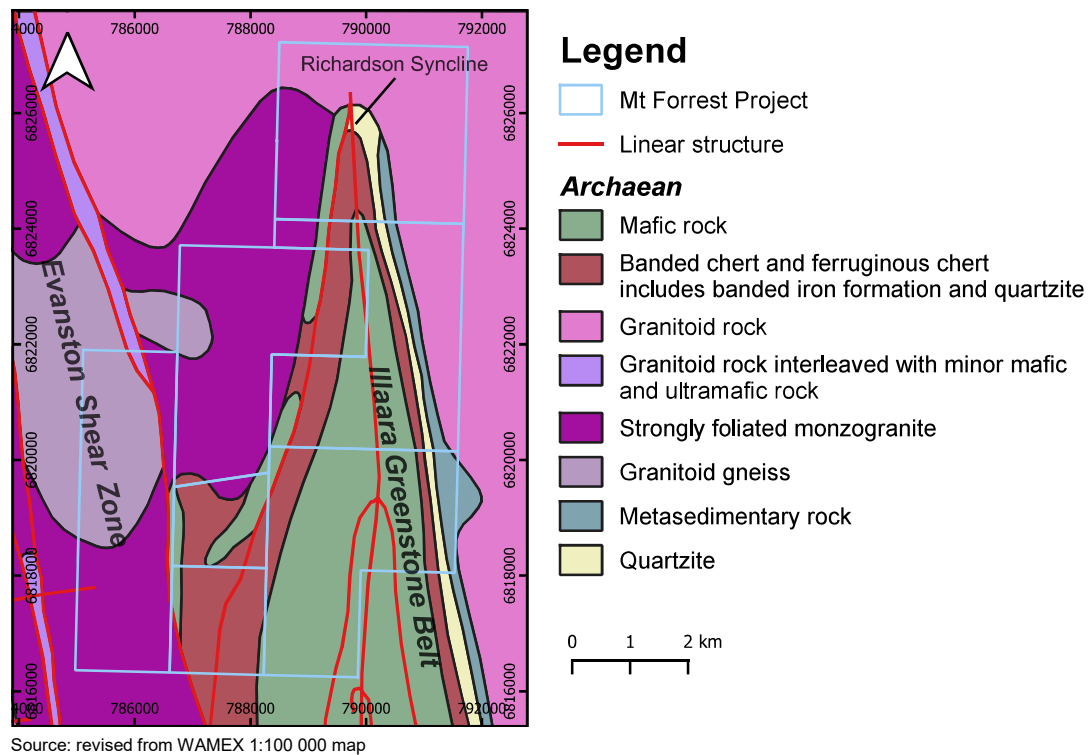
Figure 3-1: Simplified local geological map (GDA94, Zone 50)
