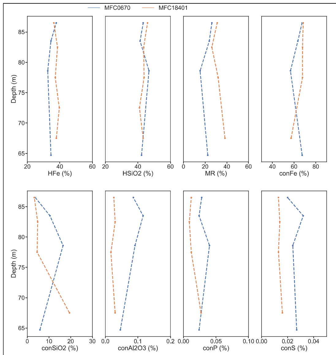
Figure 4-6: DD (blue) and RC (orange) twin pair comparison
