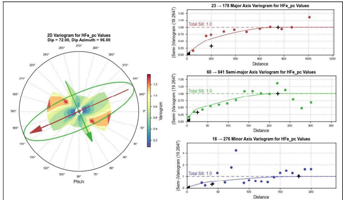
Figure 5-15: Variogram model for HFe in MF6 fresh domain
