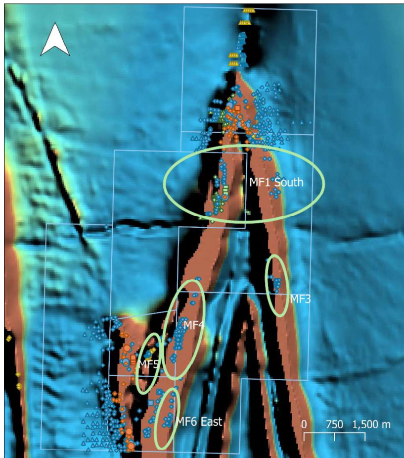
Figure 5-30: Exploration potential areas for Mt Forrest
