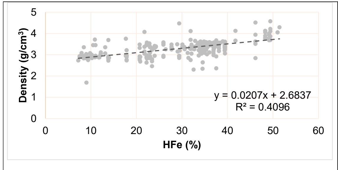
Figure 5-18: Regression plot of HFe and density
