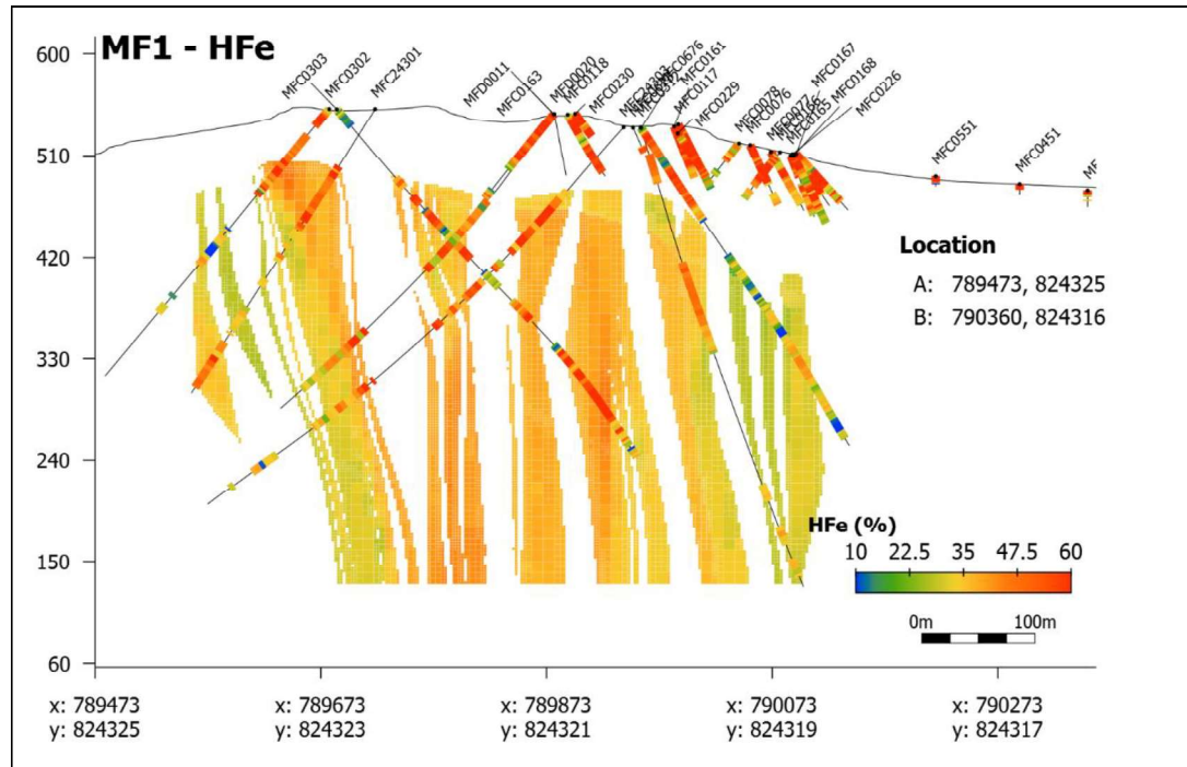
Figure 5-19: Cross section of MF1 showing HFe in blocks versus drill holes
