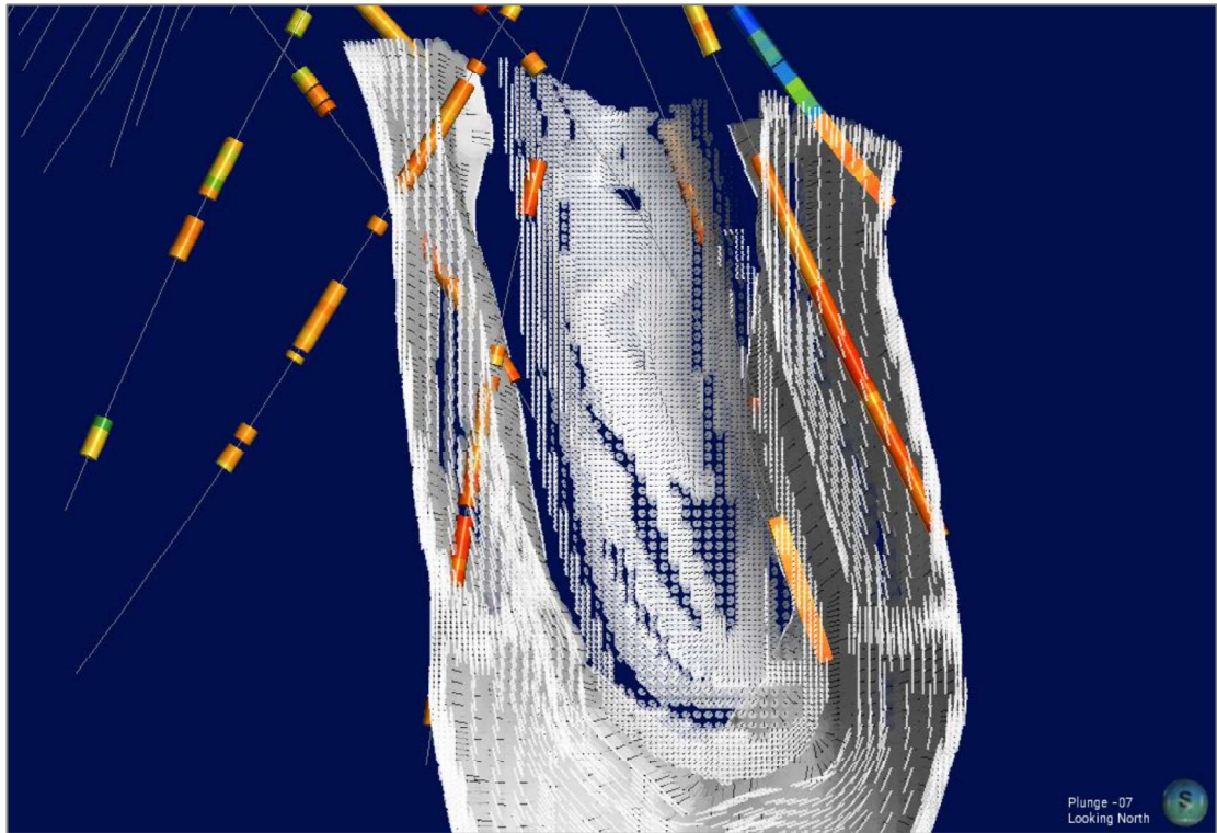
Figure 5-17: Example section showing orientation trends used for estimation in MF1
