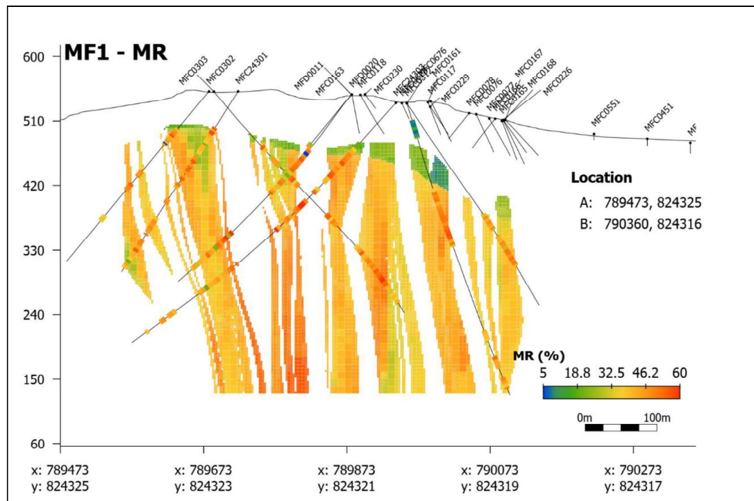
Figure 5-20: Cross section of MF1 showing MR in blocks versus drill holes
