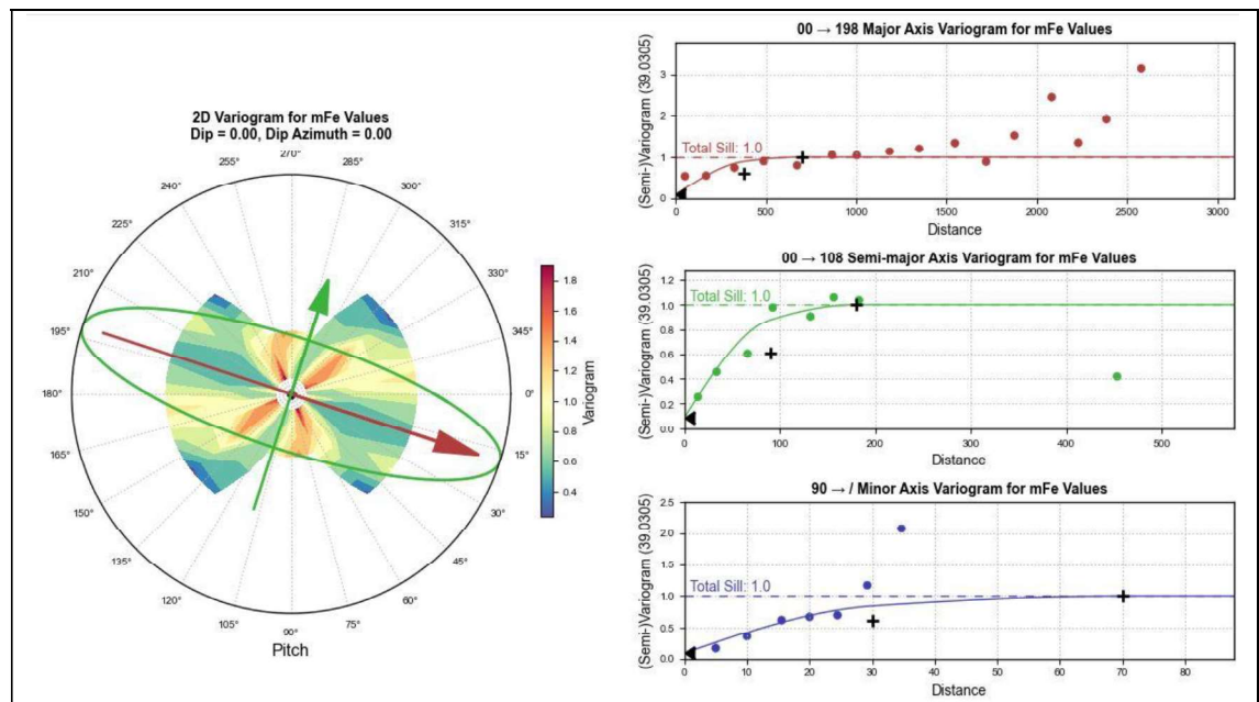
Figure 5-14: Variogram model for mFe in MF2 transition domain
