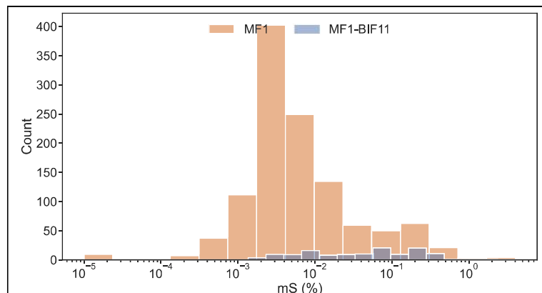
Figure 5-9: Distribution of log-transformed mS in MF1 and BIF11 lode of MF1
