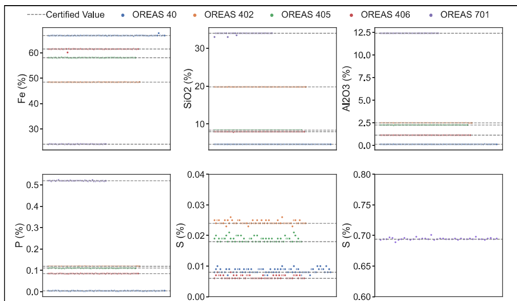
Figure 4-4: Performance of laboratory standard samples
