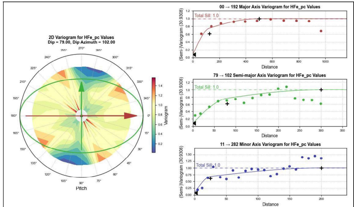
Figure 5-11: Variogram model for HFe in MF1 fresh domain
