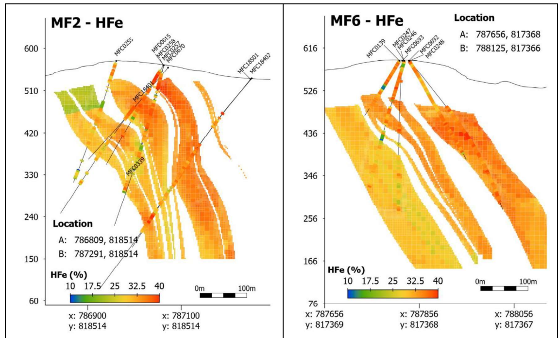
Figure 5-22: Cross section of MF2 and MF6 showing HFe in blocks versus drill holes
