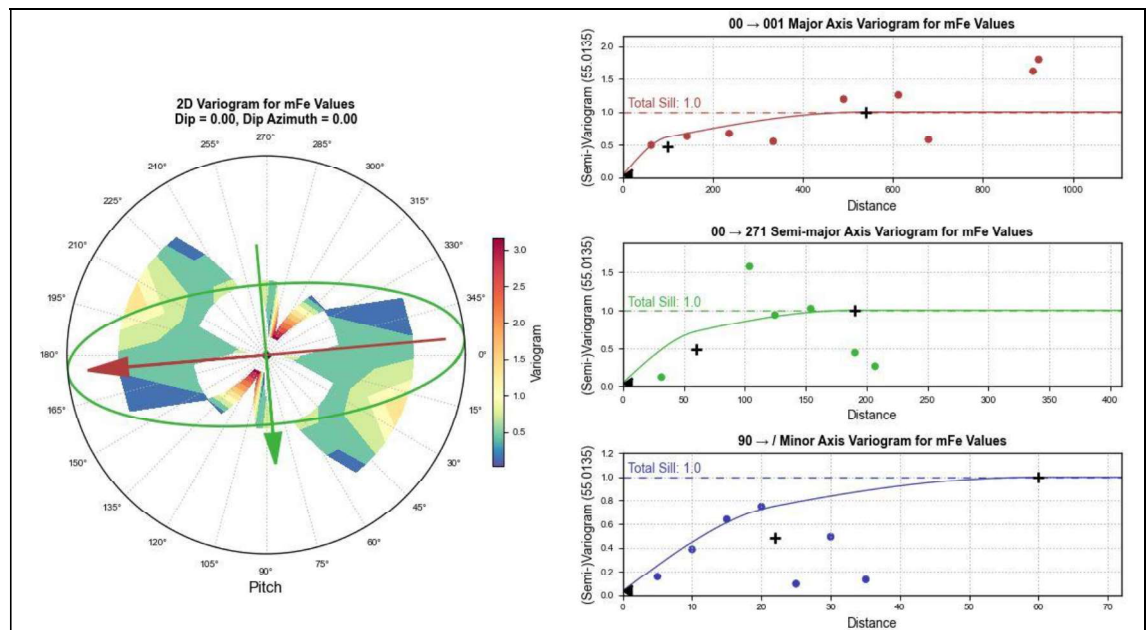
Figure 5-16: Variogram model for mFe in MF6 transition domain
