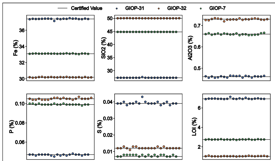
Figure 4-2: Performance of field standard samples
