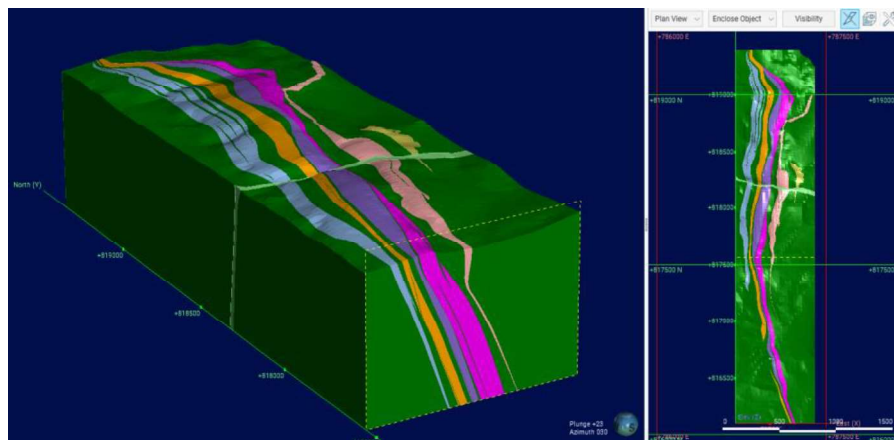
Figure 3-4: 3D model of MF2 deposit (green stands for wall rocks, other colours stand for BIF sub-domains)
