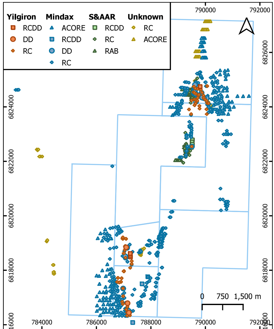
Figure 4-1: Distribution of drillholes, coloured by different periods (GDA94, Zone 50)
