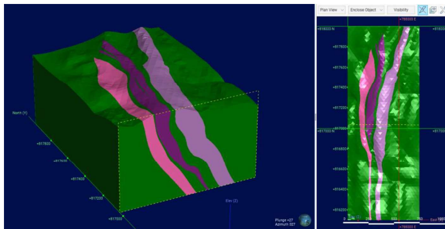
Figure 3-5: 3D model of MF6 deposit (green stands for wall rocks, other colours stand for BIF sub-domains)
