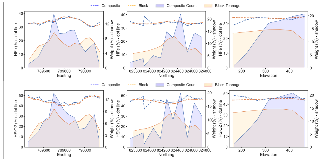
Figure 5-25: Swath plots for MF1
