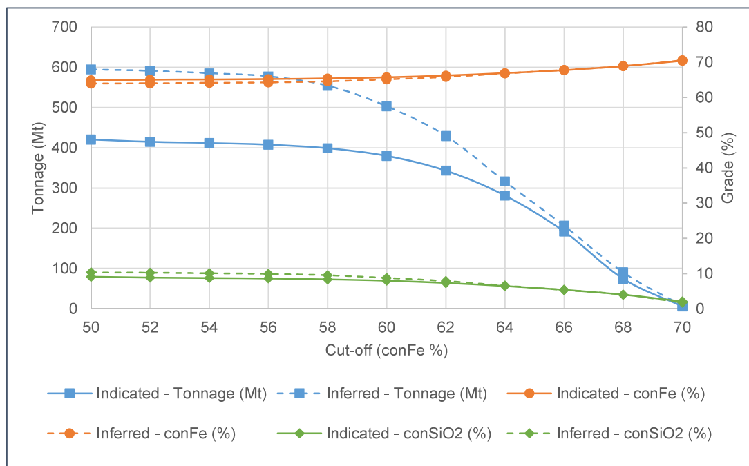
Figure 5-29: Grade-tonnage curves for conFe and conSiO 2
