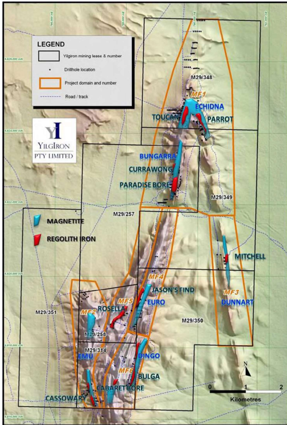
Figure 3-2: Mt Forrest magnetite domains MF1 to MF6 deposits
