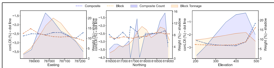
Figure 5-27: Swath plots for MF6
