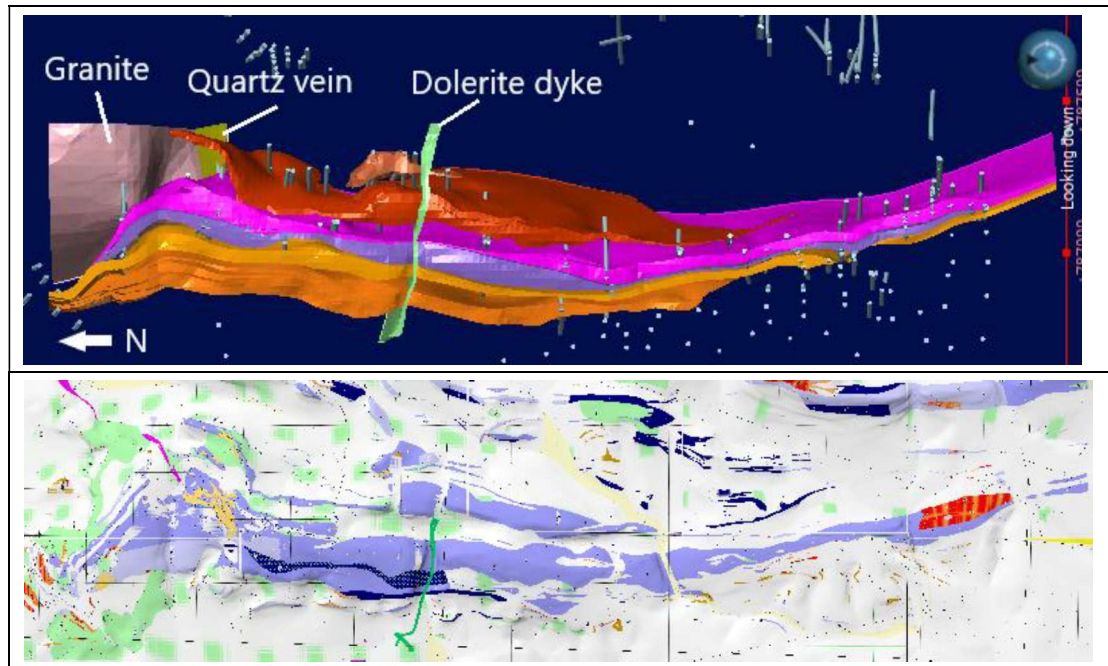
Figure 5-2: Top view of MF2 BIF model (above) and local geological map (below)
