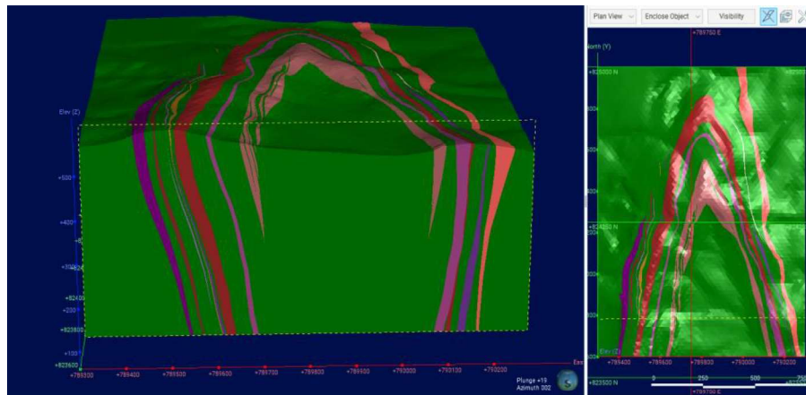
Figure 3-3: 3D model of MF1 deposit (green stands for wall rocks, other colours stand for BIF sub-domains)
