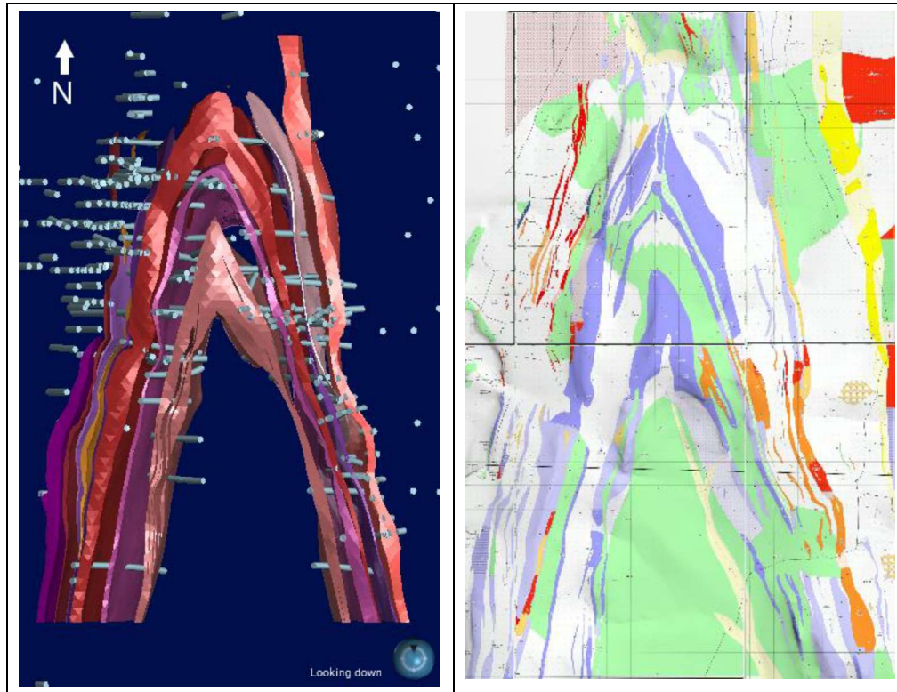
Figure 5-1: Top view of MF1 BIF model (left) and local geological map (right)
