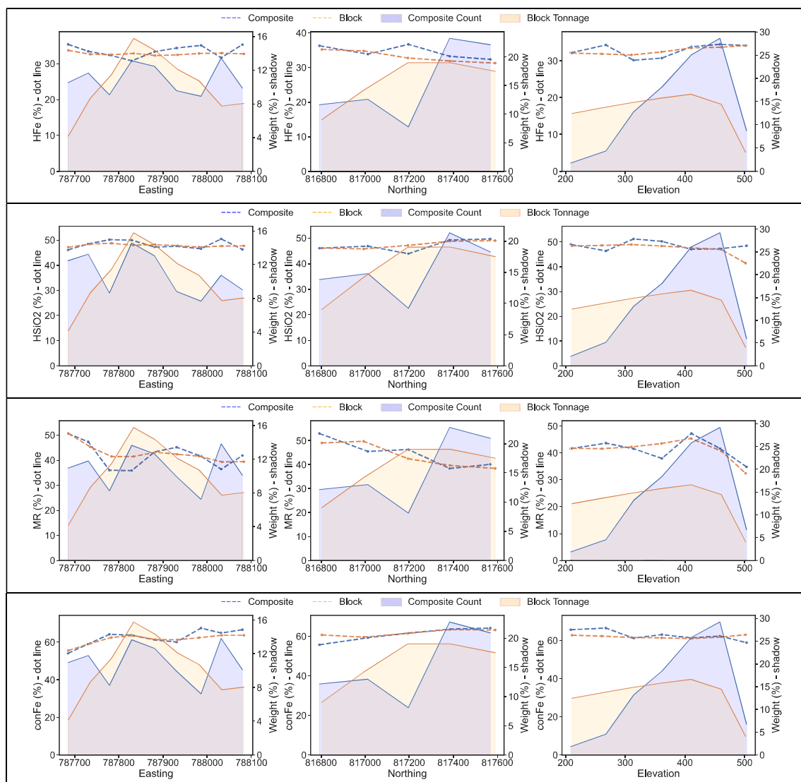
Figure 5-27: Swath plots for MF6
