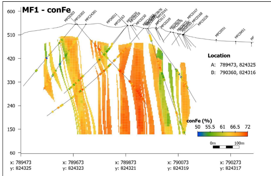
Figure 5-21: Cross section of MF1 showing conFe in blocks versus drill holes
