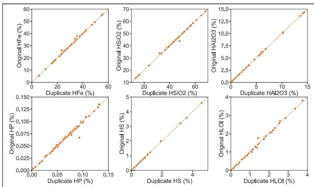
Figure 4-5: Performance of laboratory duplicate samples
