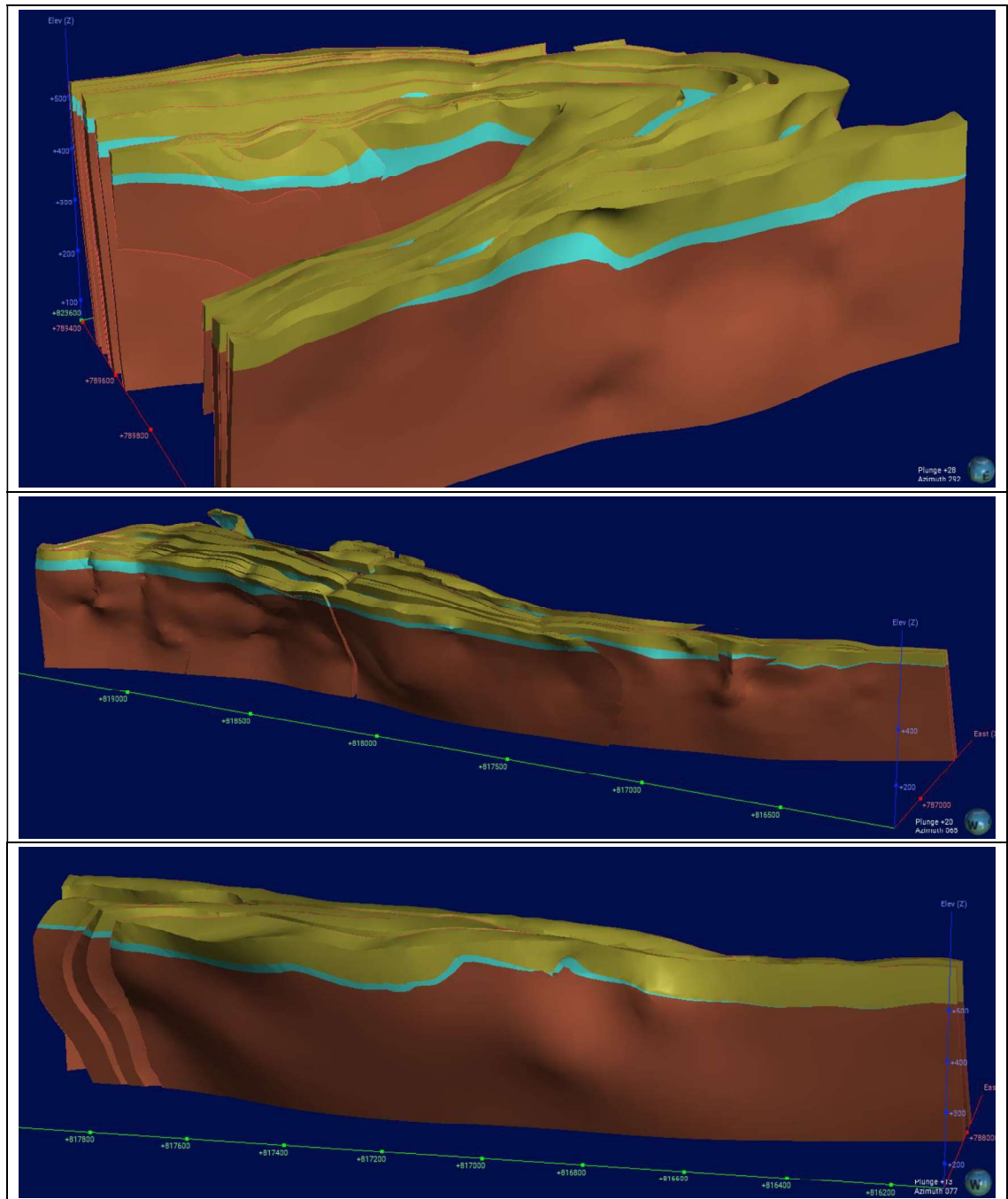
Figure 5-4: 3D view of oxide (yellow), transition (azure), and fresh (brown) domains for MF1 (top), MF2 (middle), and MF6 (bottom)
