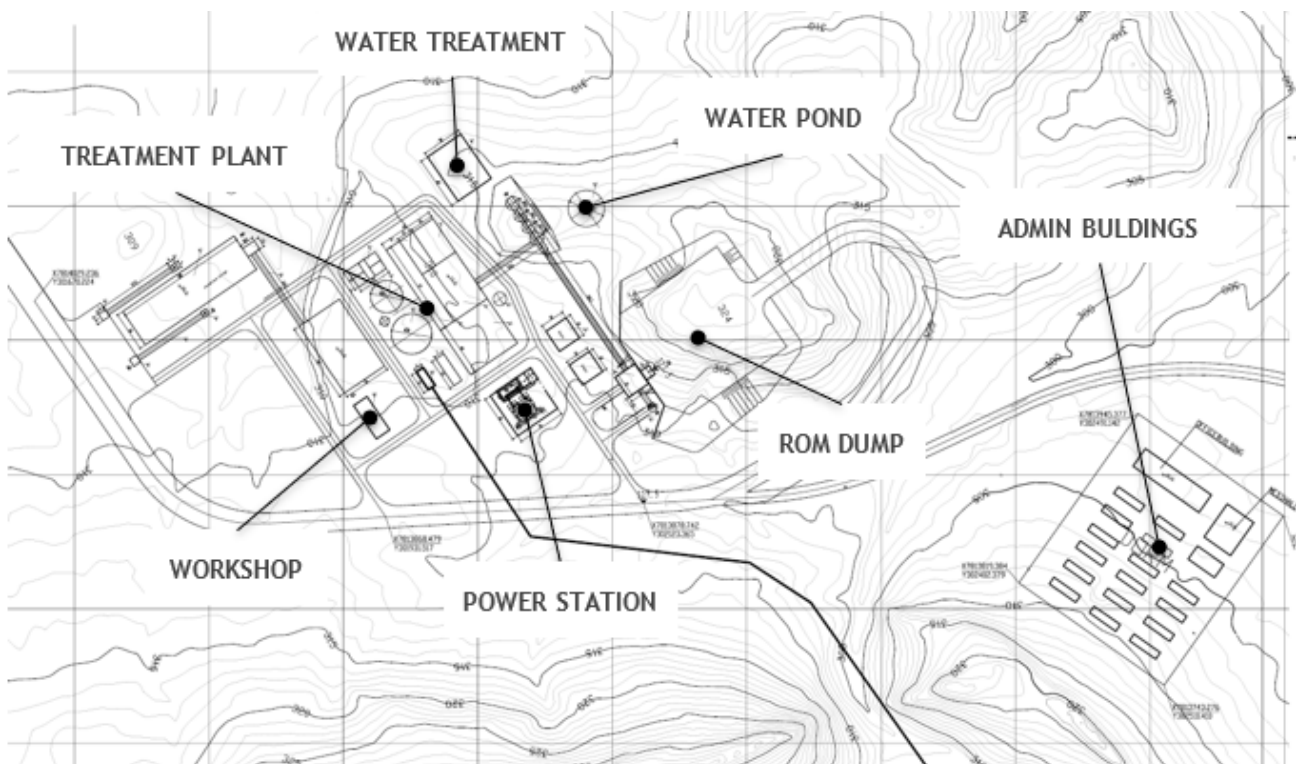
Figure 9-1: Site Layout
