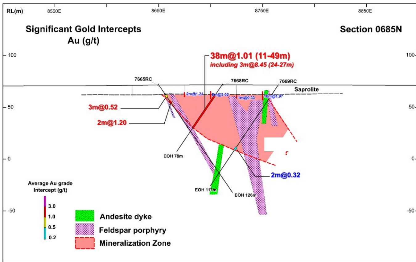
Figure 1 above: Section 0685N showing the near surface ore zone close to the Chatree Gold Mine.
