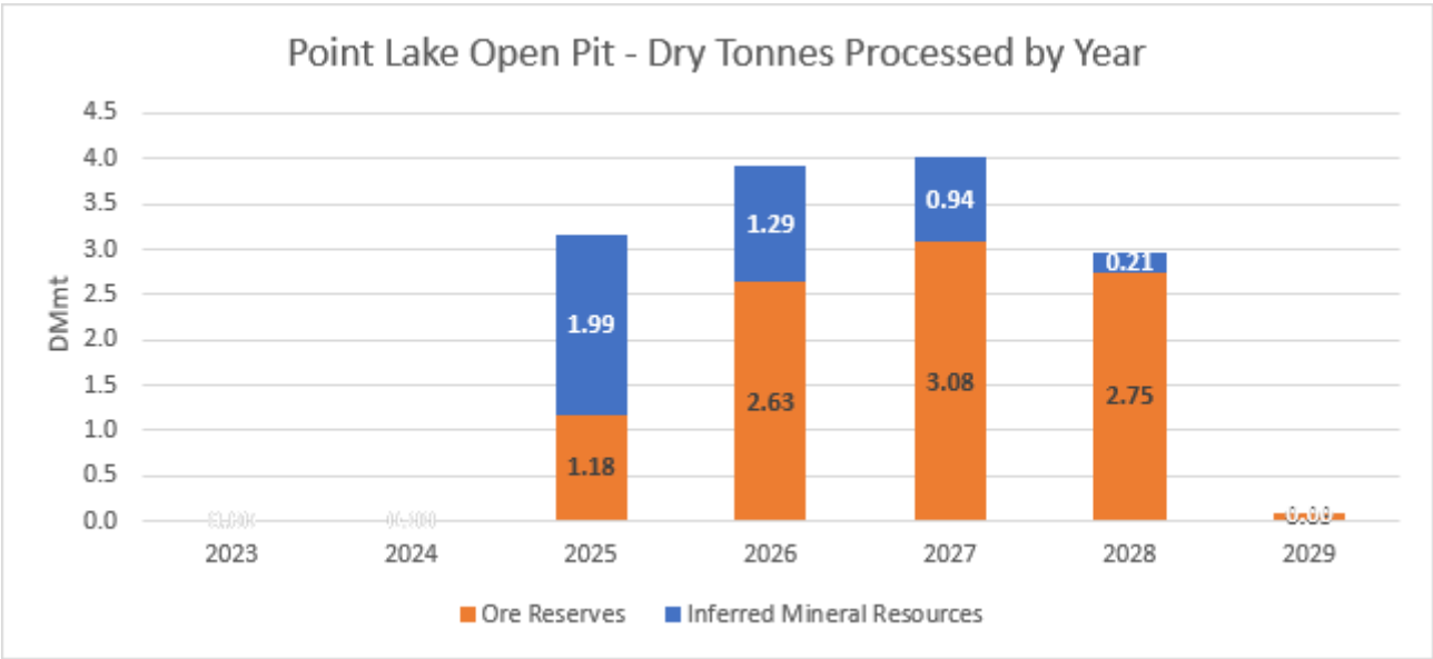
Figure 3.23 – Production profile for Point Lake
