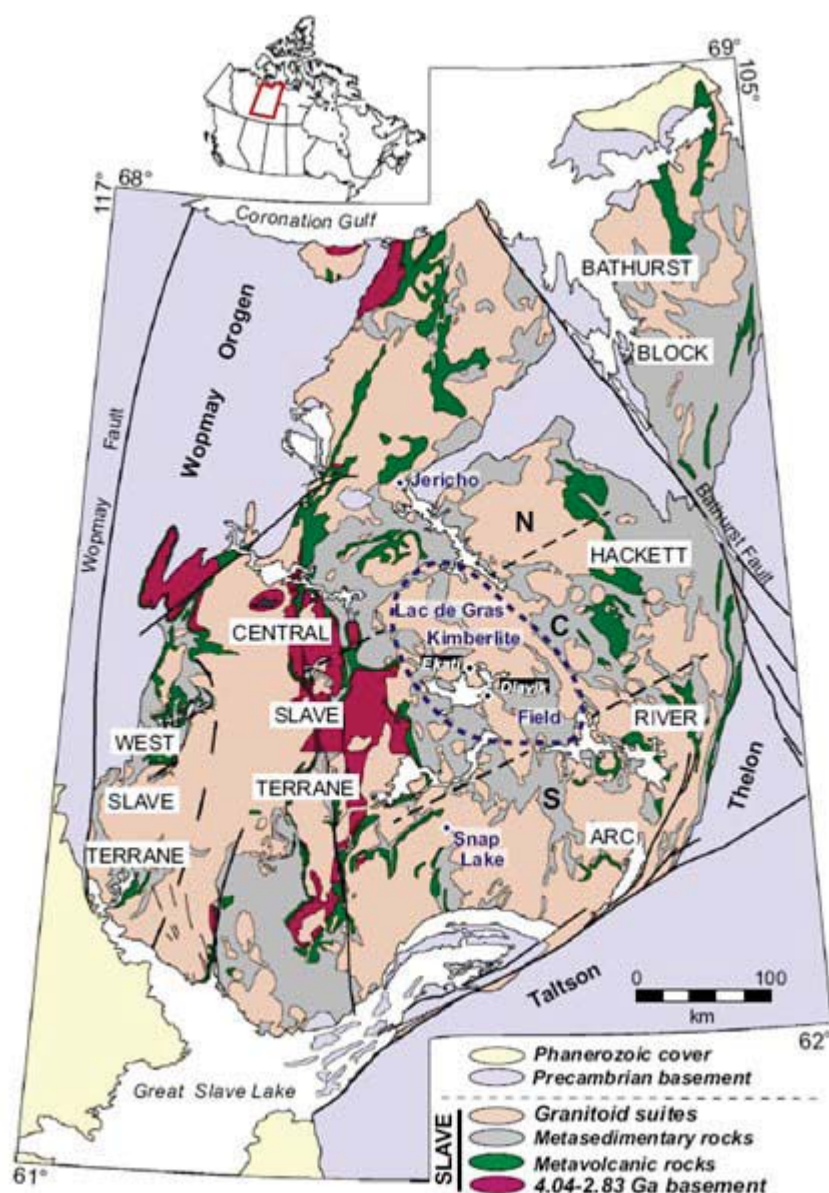
Figure 5-1: Geological map of the Slave craton
