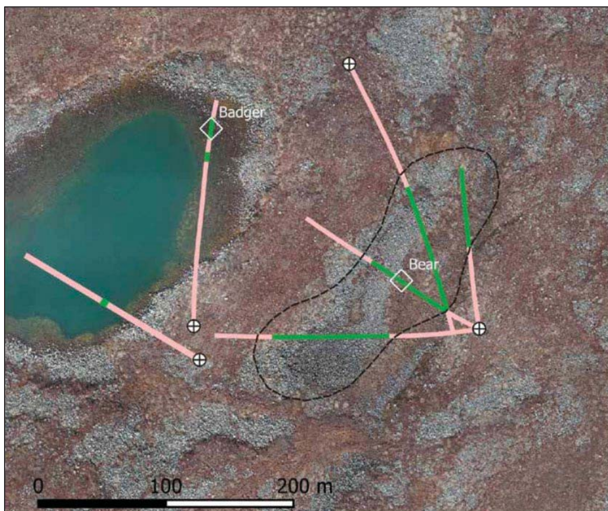
Figure 6-4: Projected core holes drilled in the vicinity of the Bear and Badger kimberlites Note: The drill traces are colour coded by generalised rock type (green = kimberlite; pink = granite). A preliminary interpretation of the outline of the Bear kimberlite at surface (based on drill results and geophysics) is shown.
