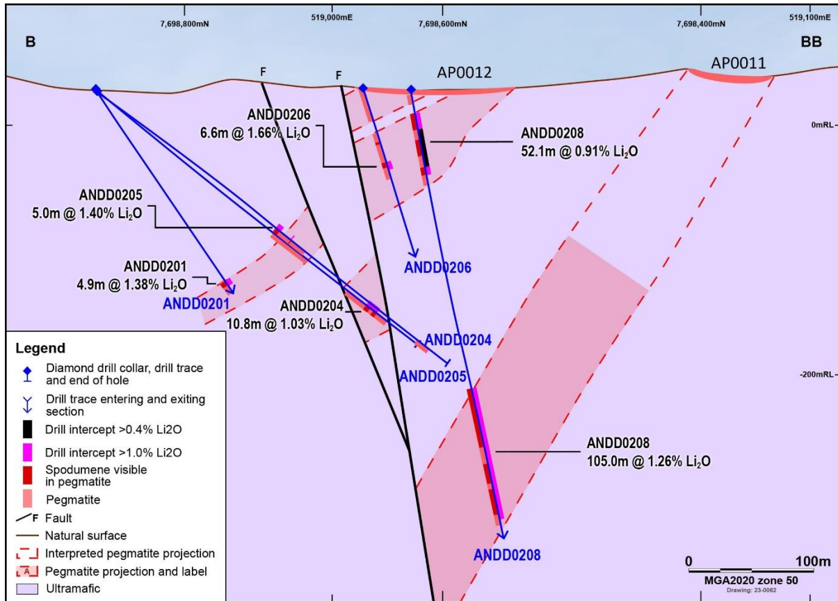
Figure 3: Section B-B through AP0011 / AP0012 pegmatites with reported lithium intersections
