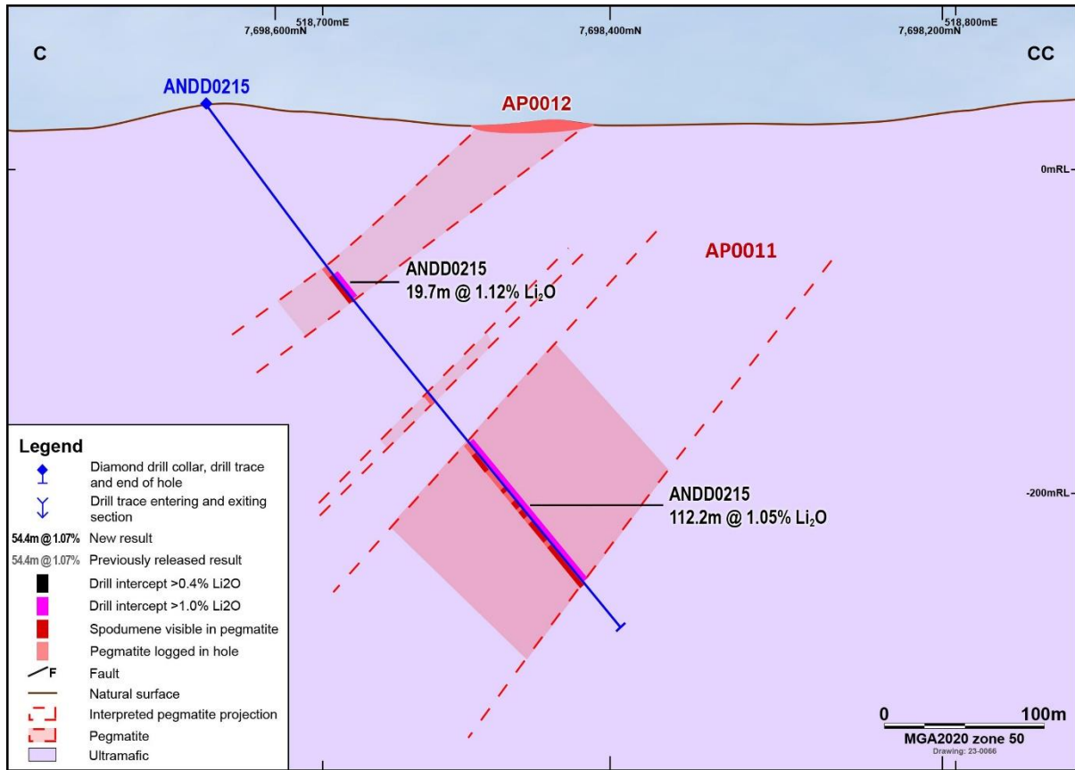
Figure 5: Section C-CC through AP0011 / AP0012 pegmatites with reported lithium intersections
