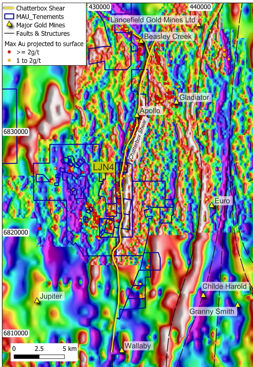
Figure 3. The Lady Julie North 4 Chatterbox Interpreted Shear shown on a Gravity image with major gold deposits.
