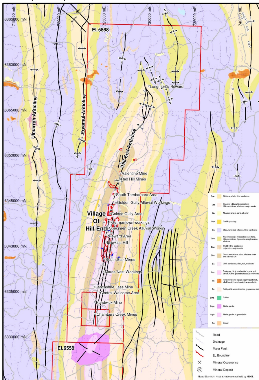
Image 2: Local Geology
