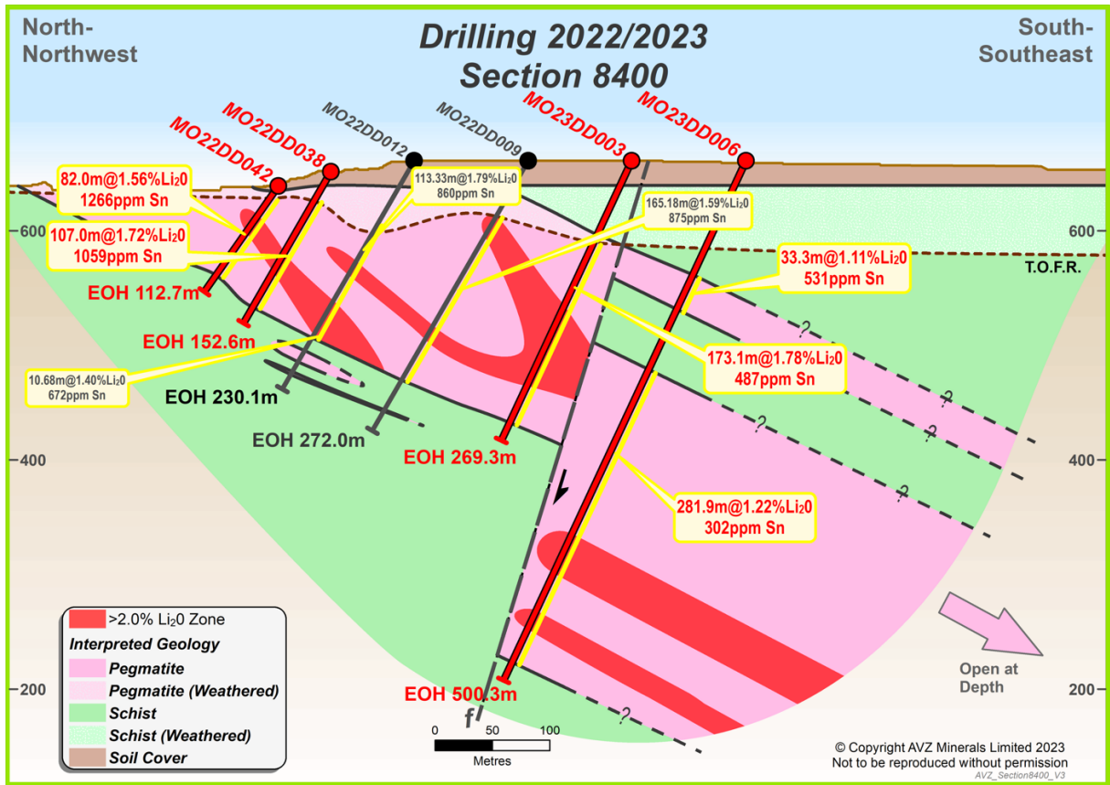
Figure 11: Intersections on section 8,400mN
