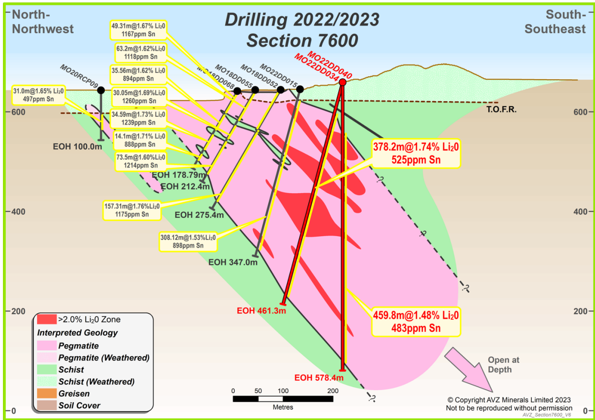
Figure 3: Intersections on section 7,600mN
