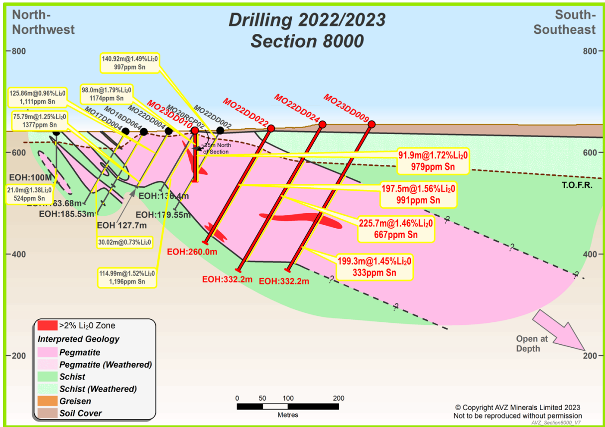
Figure 7: Intersections on section 8,000mN
