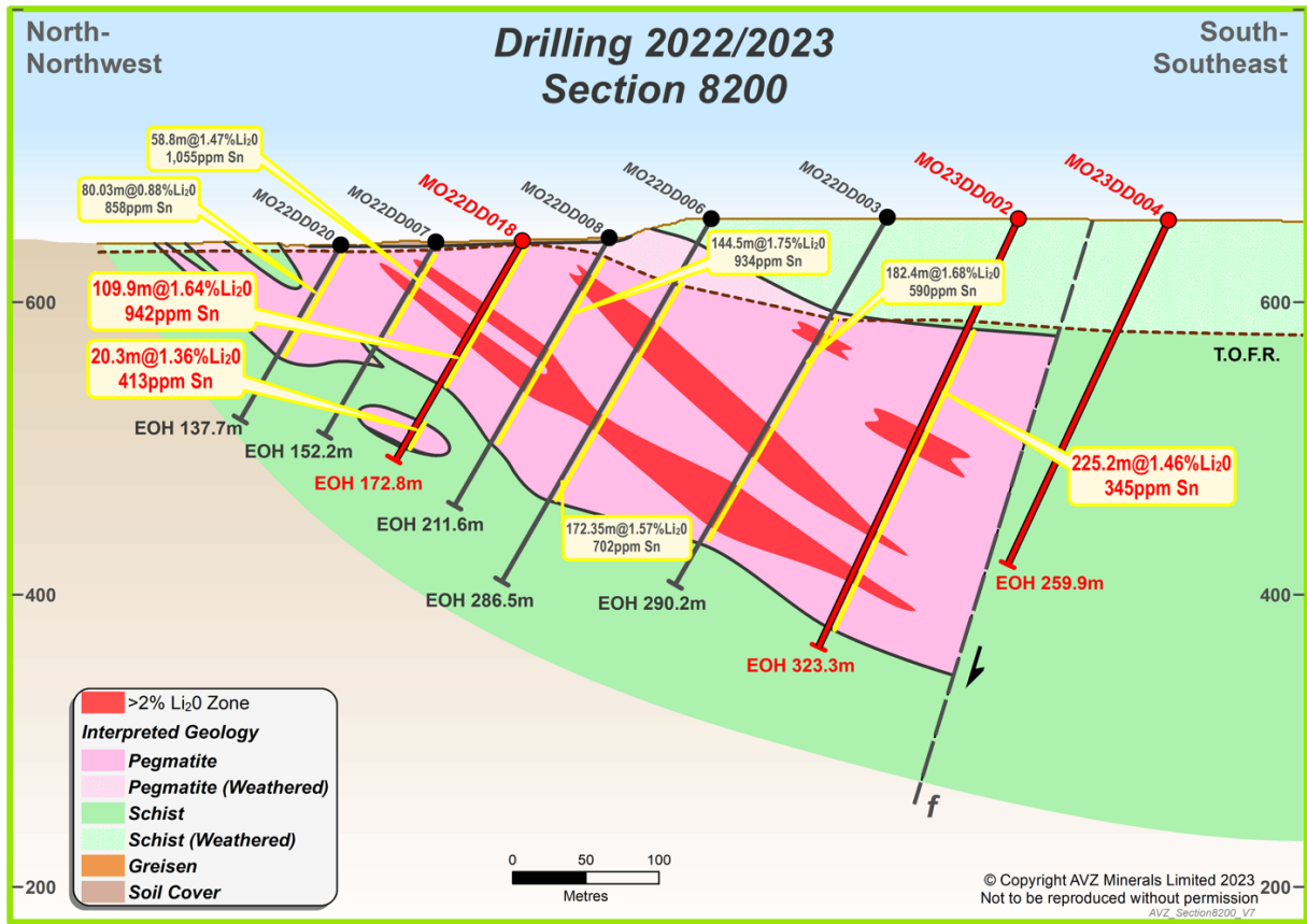
Figure 9: Intersections on section 8,200mN
