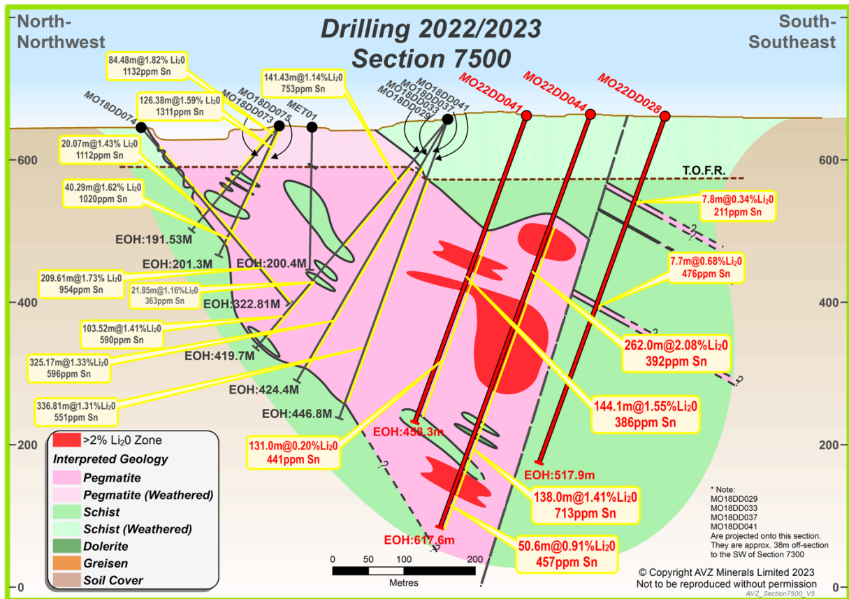
Figure 2: Intersections on section 7,500mN
