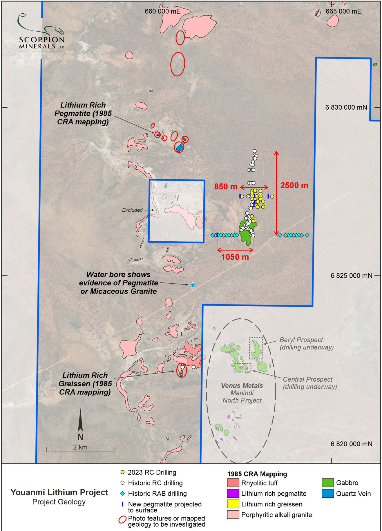
Figure 7: Local Outcrop Geology
