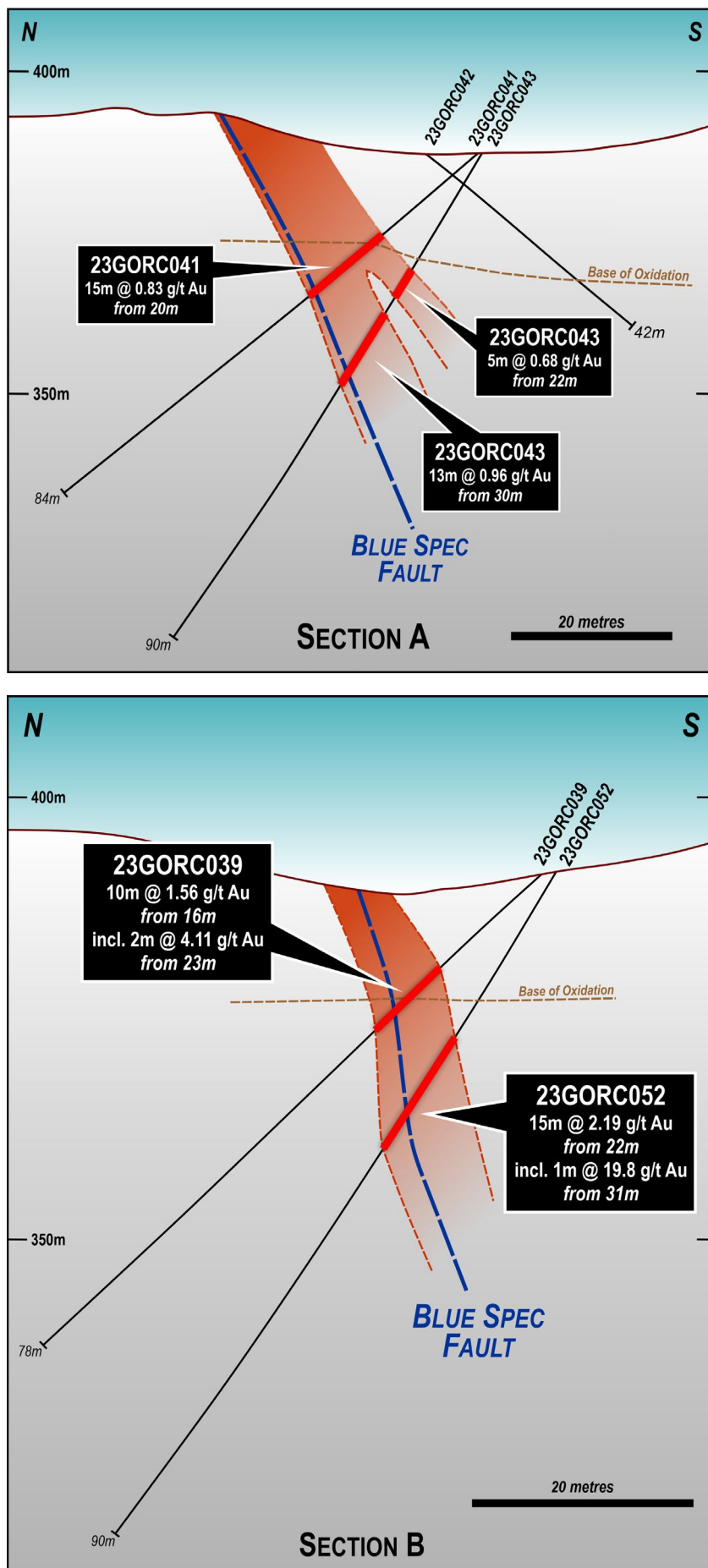
Figure 2 – Cross-sections through the recent drilling at Felix east with interpreted zones of mineralisation >0.5g/t Au.
