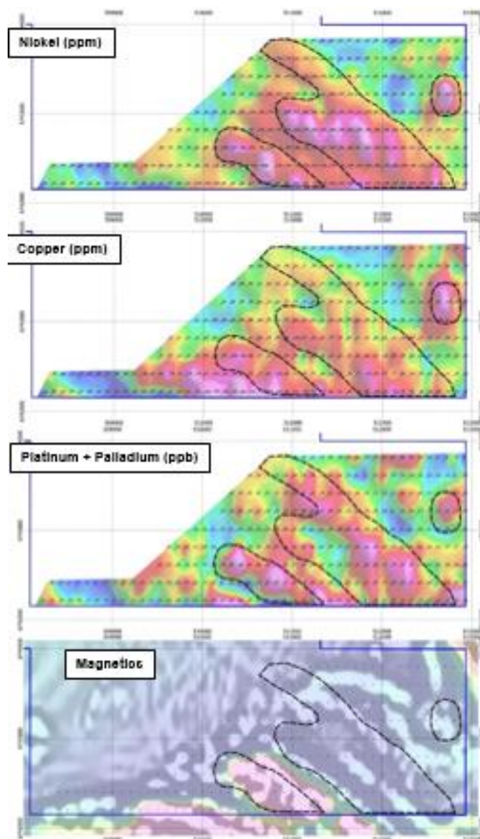
Figure 4A (top) colour gridded Ni-in-soil image. Figure 4B (second top) colour gridded Cu-in-soil image. Figure 4C (third from top) colour gridded Pt+Pd-in-soil image. Figure 4D (bottom) Airborne magnetic MrtpcMrtplap image showing and soil anomalies.
