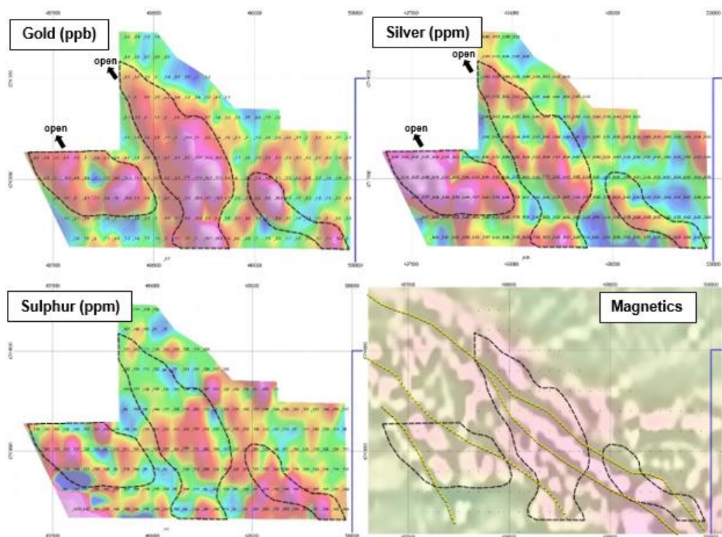
Figure 3A (top left) colour gridded Au-in-soil. Figure 3B (top right) colour gridded Ag-in-soil. Figure 3C (bottom left) colour gridded S-in-soil. Figure 3D (bottom right) Airborne magnetic MrtpcMrtplap showing interpreted lineaments (yellow dash) and soil anomalies.
