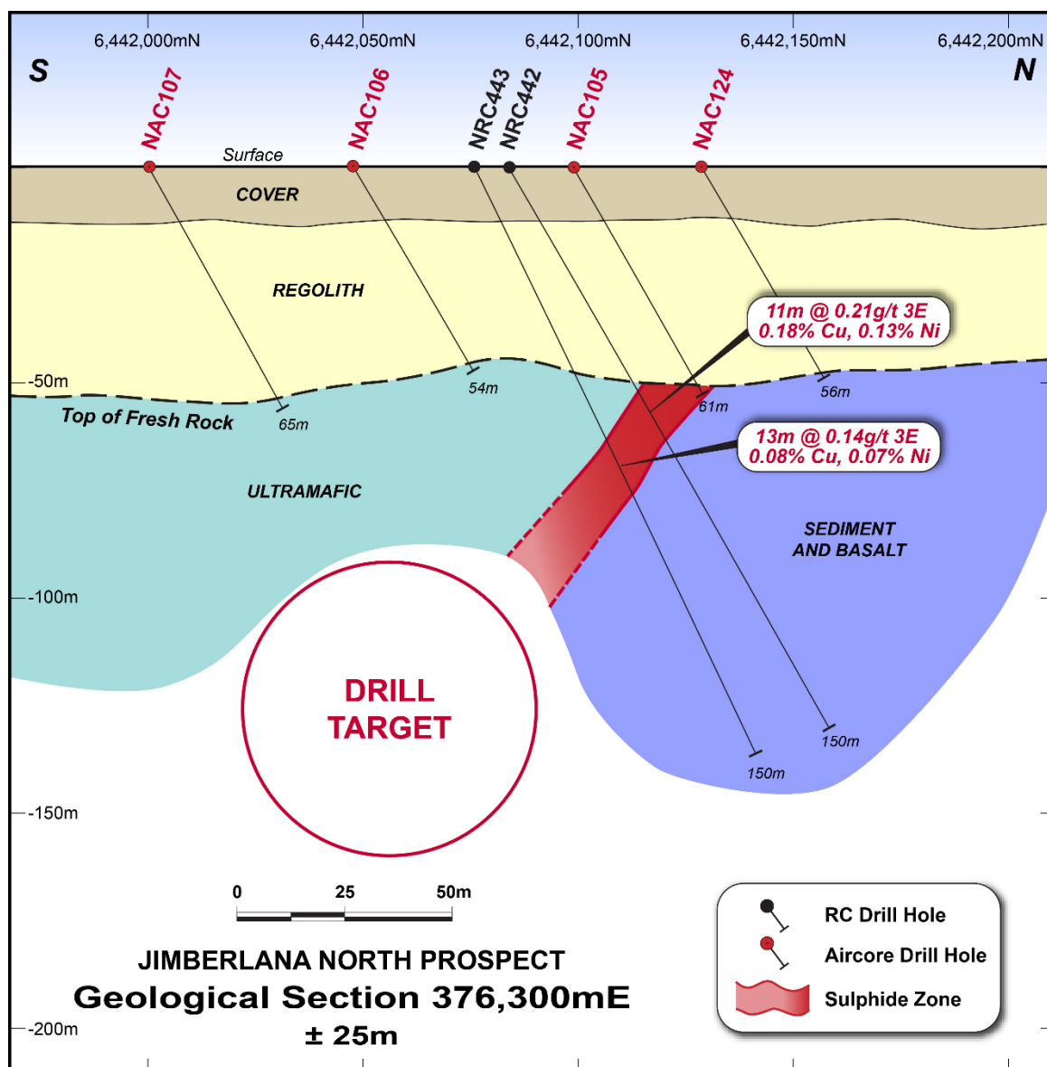
Figure 2 – Jimberlana North section 376,300E showing sulphide target for drill testing
