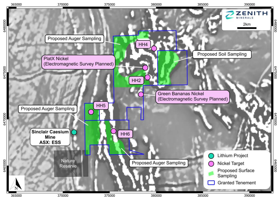
Figure 5: Hayes Hill Project – Nickel Targets and Proposed Work
