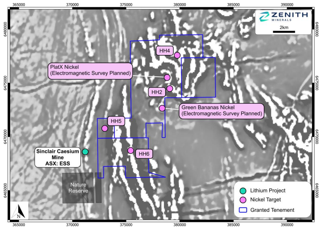
Figure 4: Hayes Hill Nickel Targets and Planned EM Surveys
