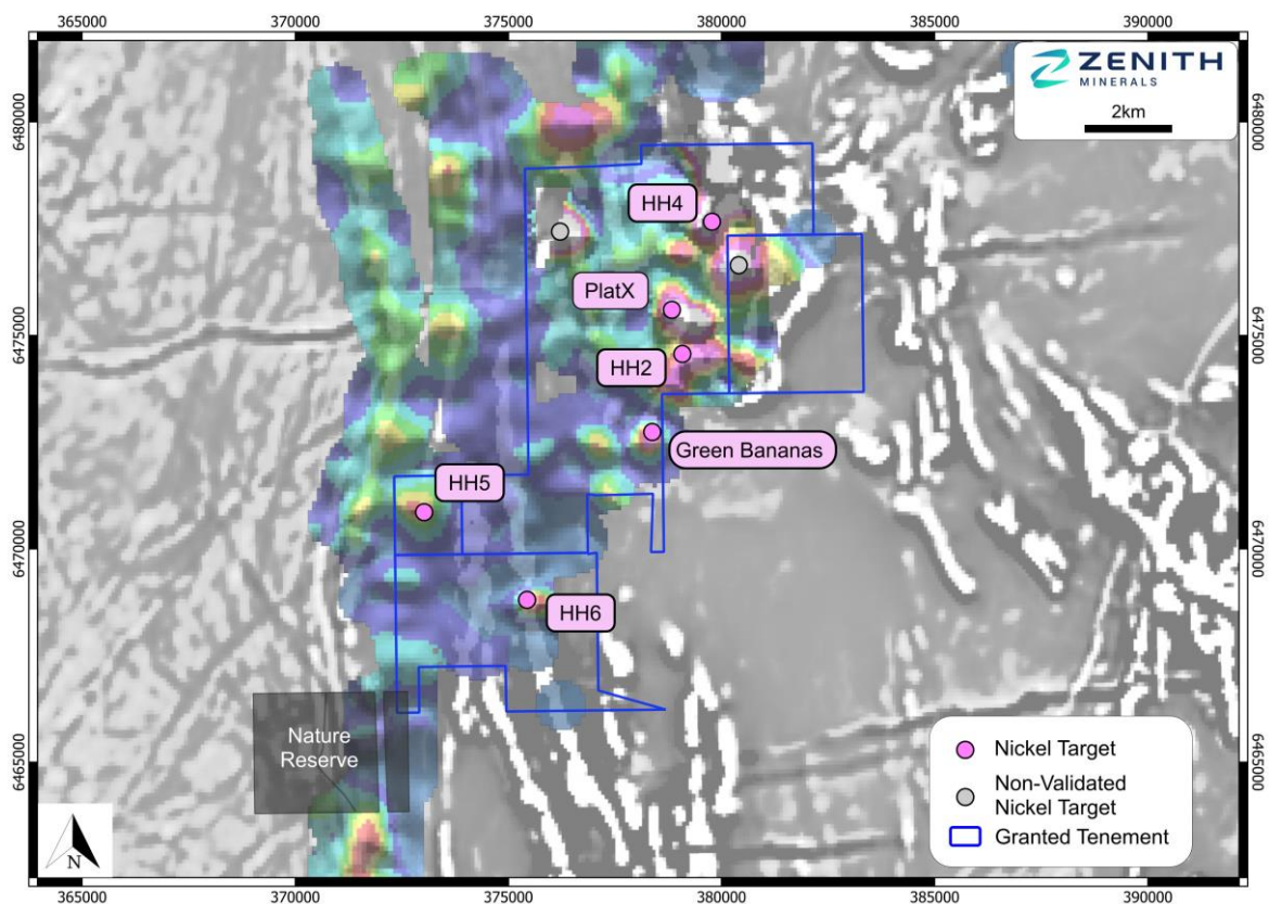
Figure 3: Hayes Hill Nickel Targets
