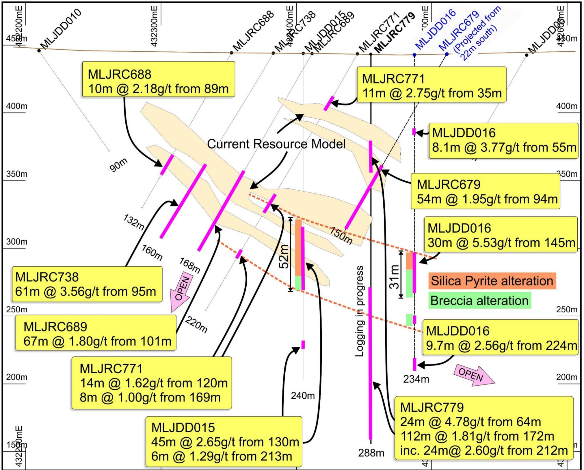
Figure 1. Composite cross section for LJV4 centre area showing thickened high-grade dipping gold zone containing breccia and silica-pyrite alteration, upper mineralised zone, older resource model outline, new drill hole MLJRC779 and potential depth extensions at depth, downdip to the east and south.
