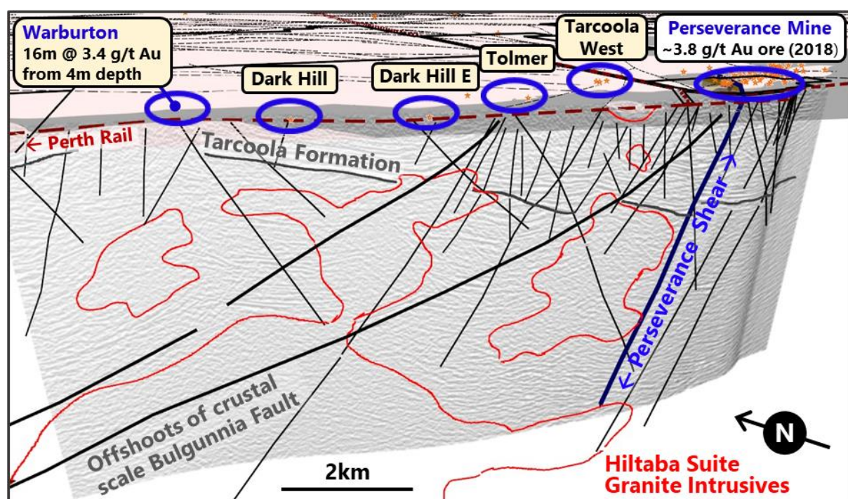
Fig 1 – Tarcoola Structural Architecture Interpreted from Seismic Reprocessing (2020) 1
